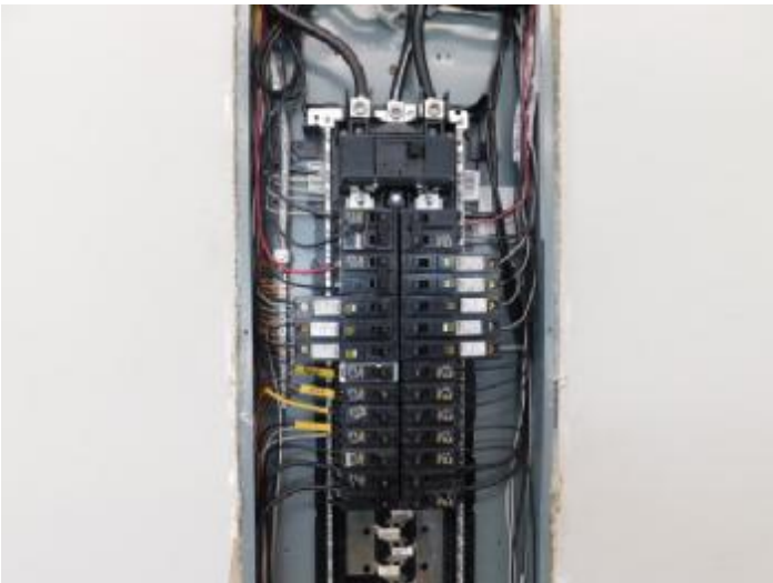
Electric panel
