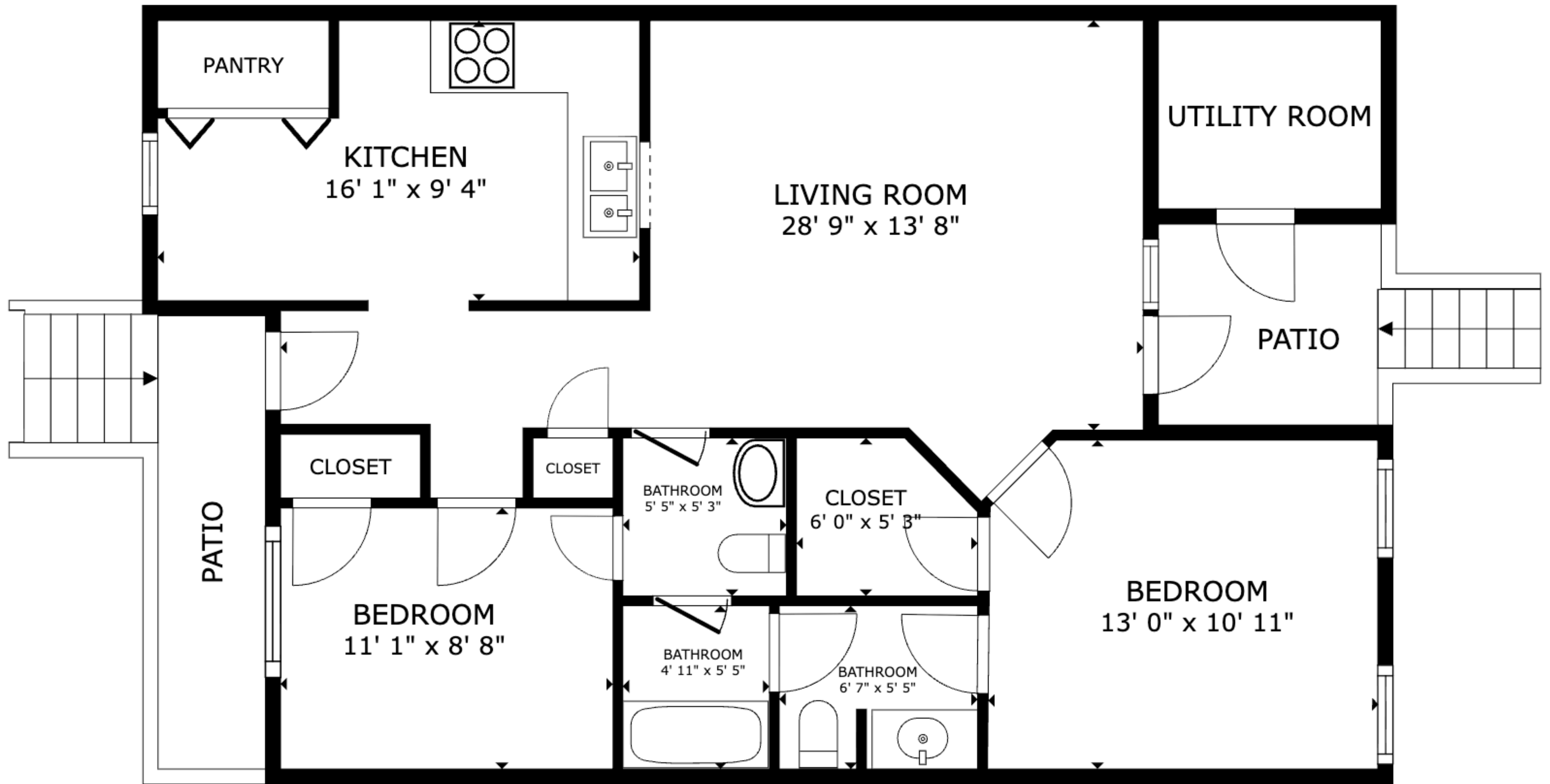
FLOOR PLAN
