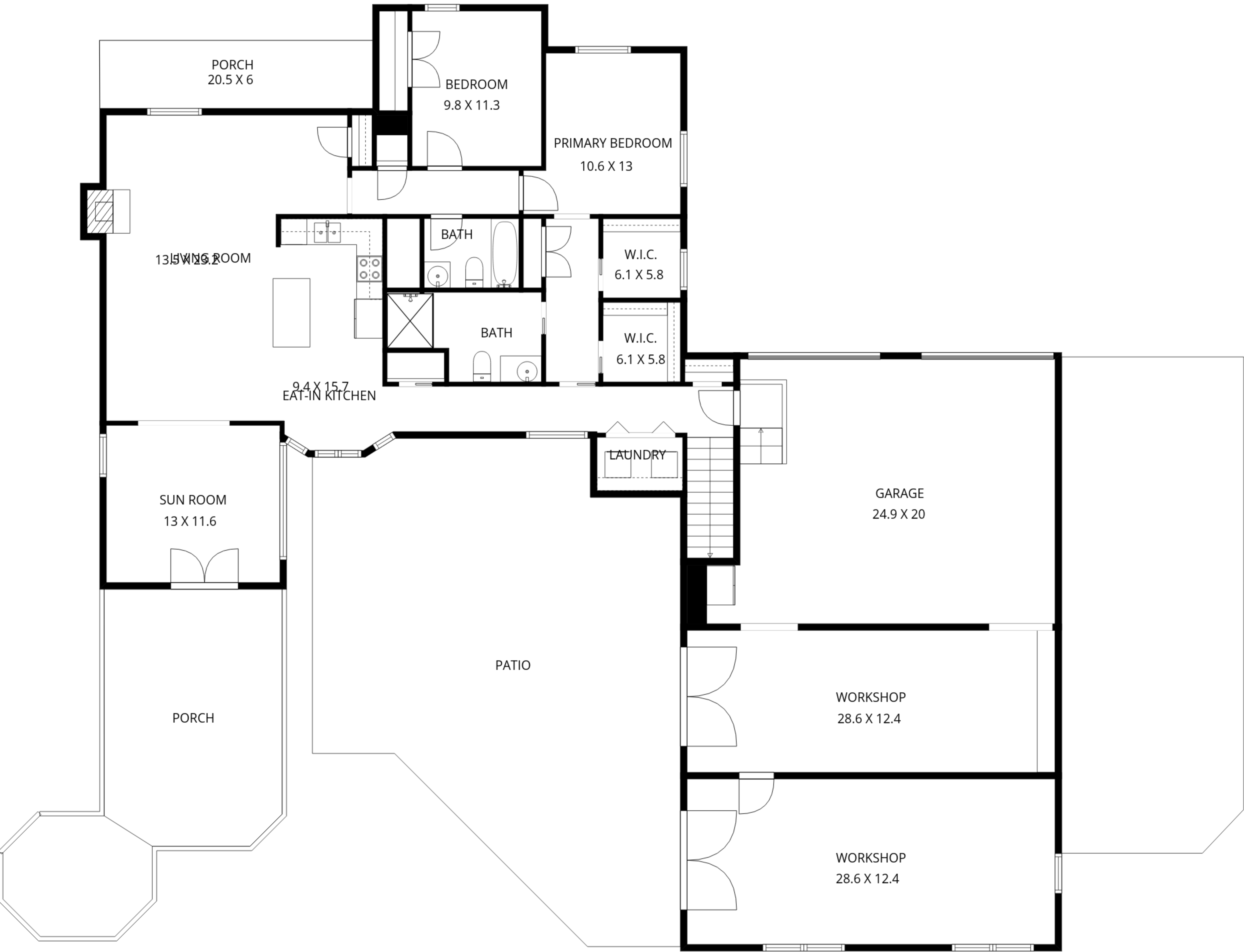
1ST FLOOR
