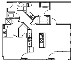
12.1 B2-6.1 UNIT PLAN - 1120 SF SCALE: 1/8" = 1'-0"
