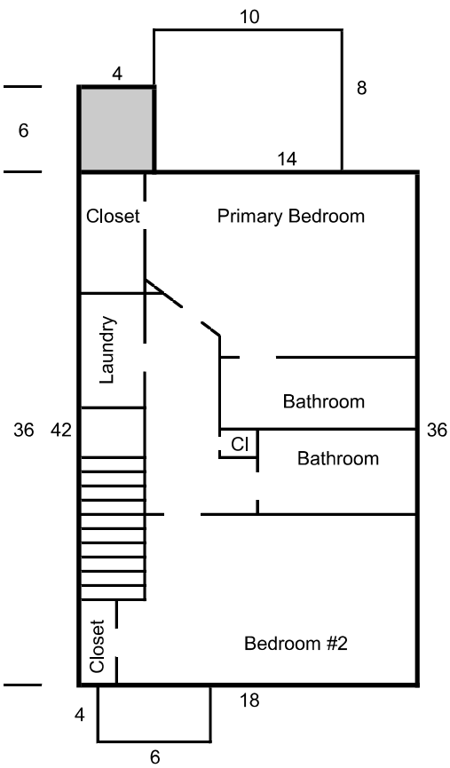
2nd Level
