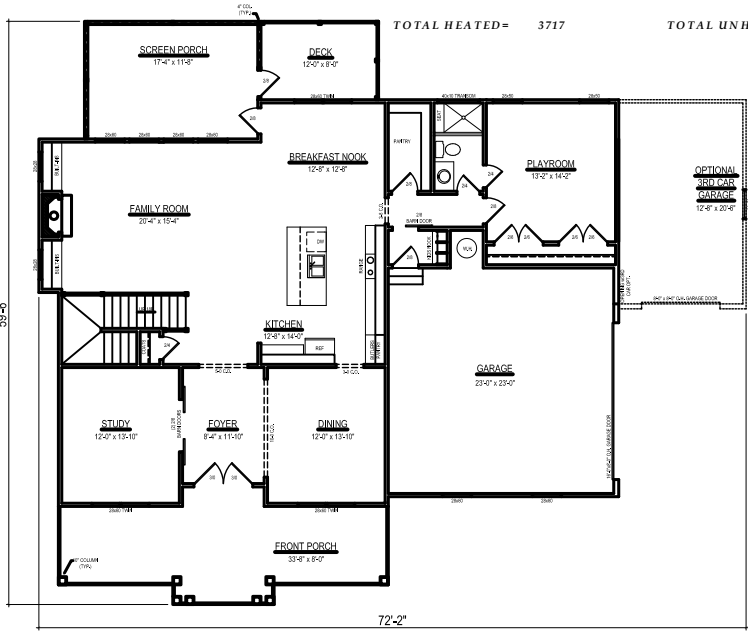
FIRST FLOOR PLAN CEILING HT. = 10'-0"
