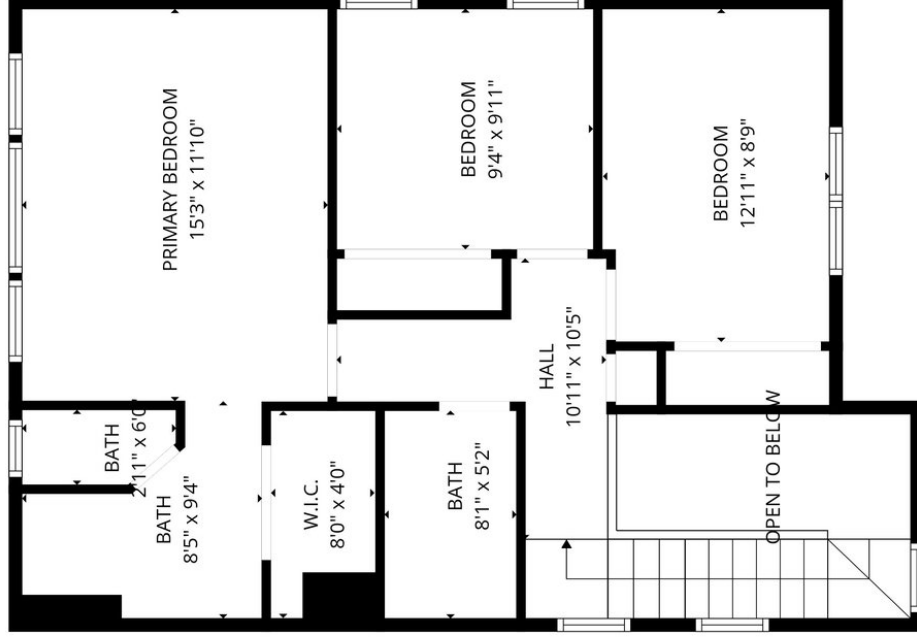
2nd floor
