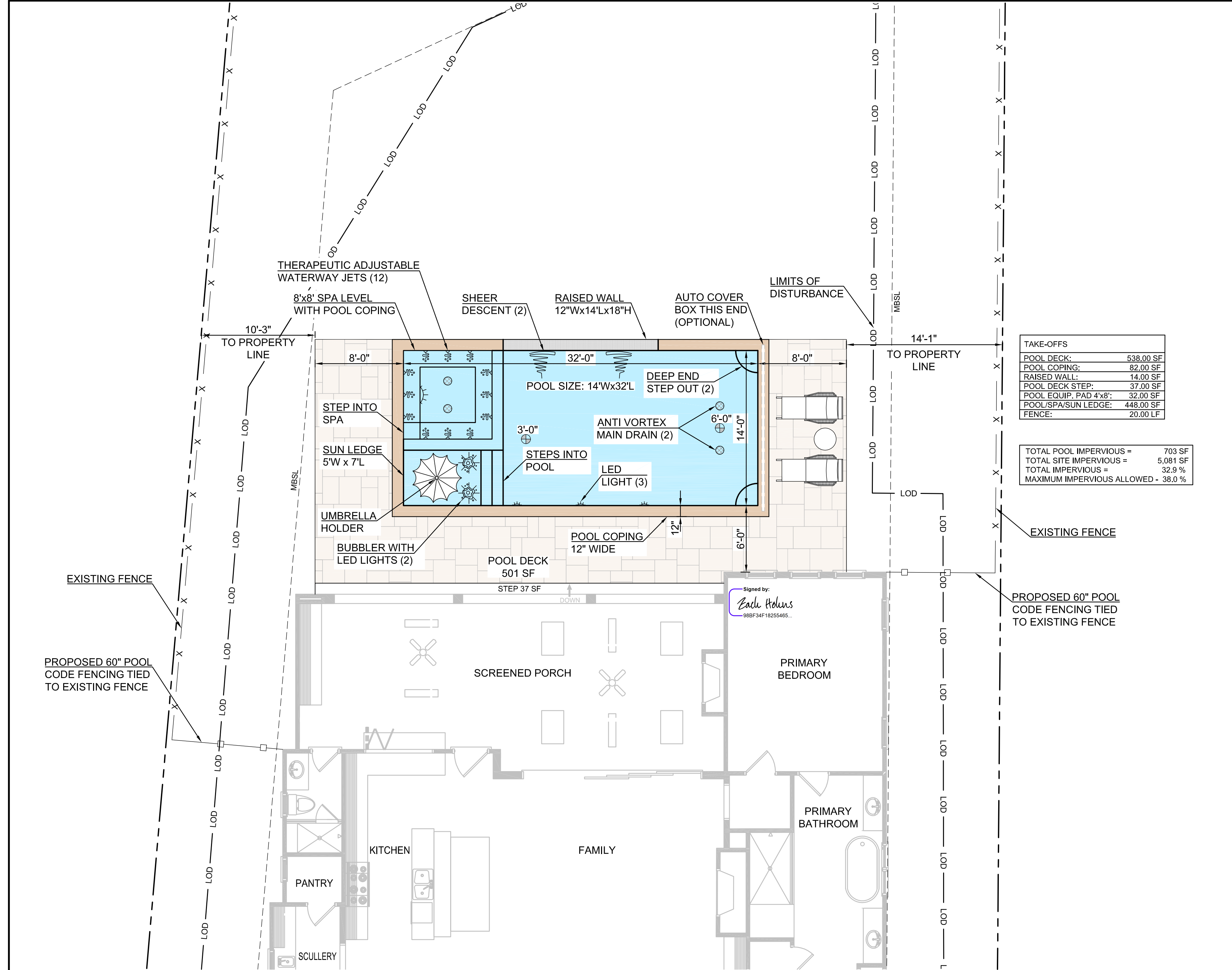
1 PRELIMINARY LUXURY POOL DESIGN 0 12 SCALE: 3/16"=1'-0"
