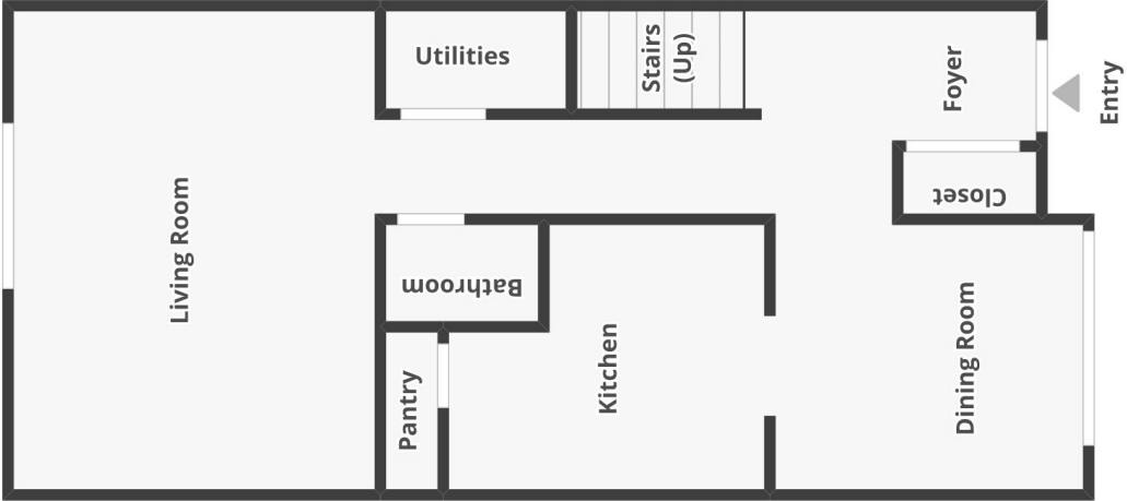
FLOOR 1
