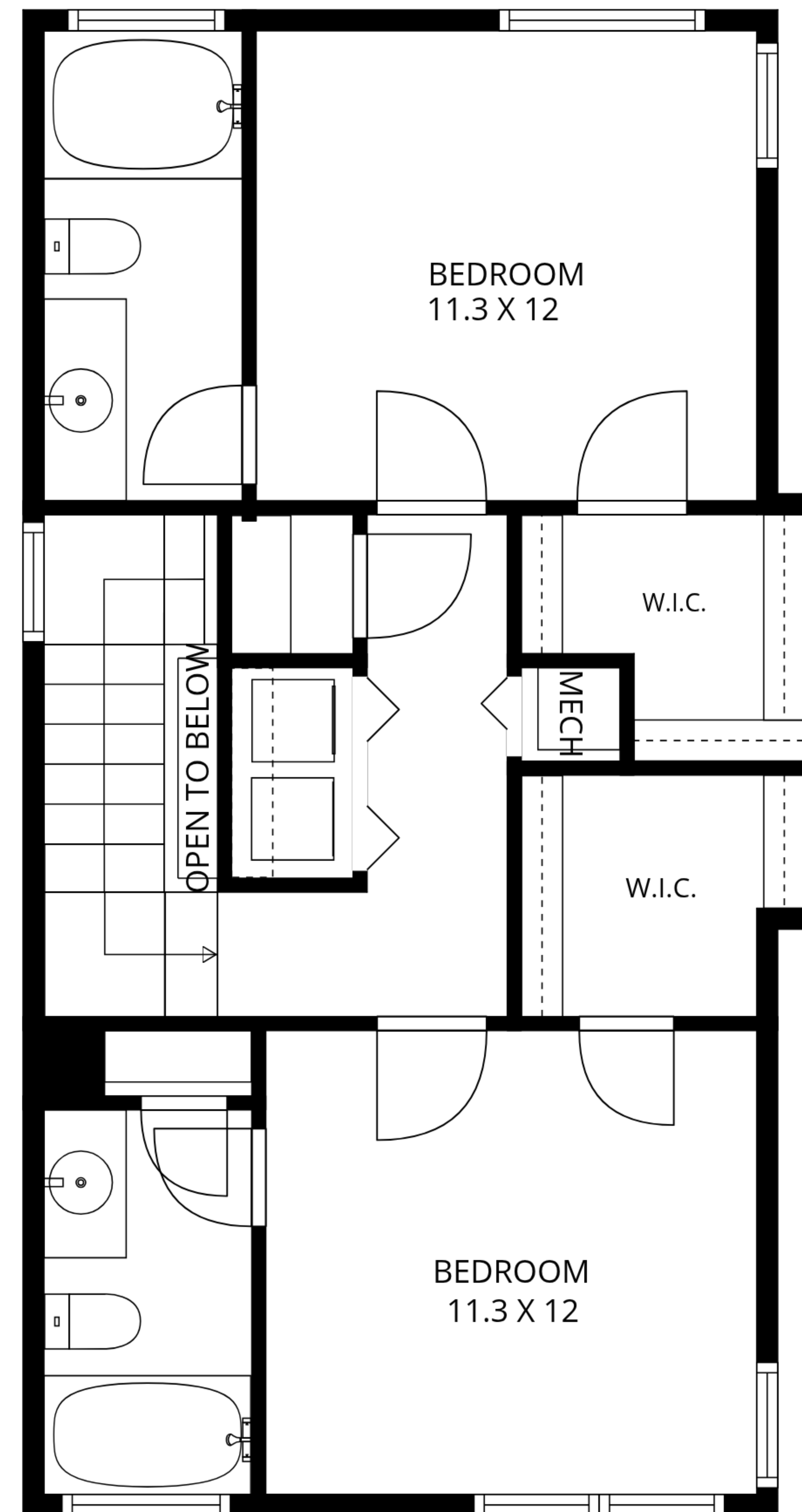
2ND FLOOR
