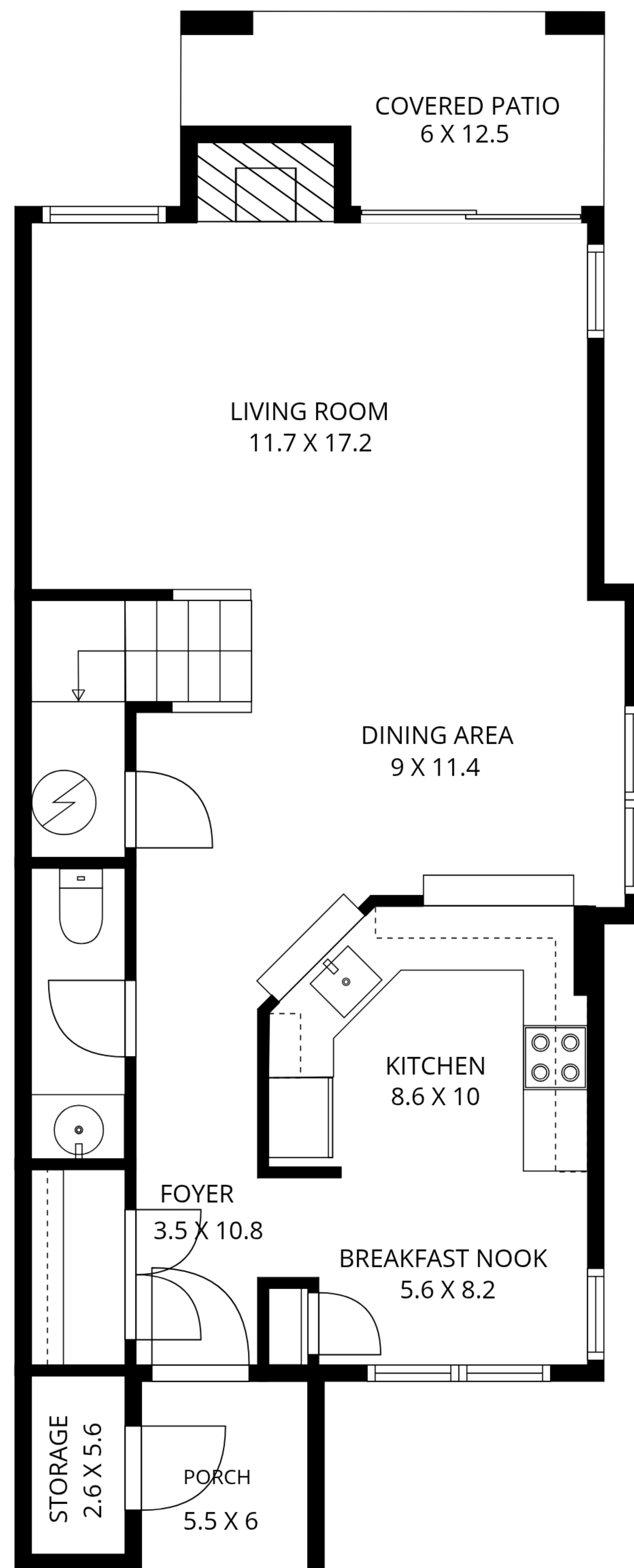
1ST FLOOR
