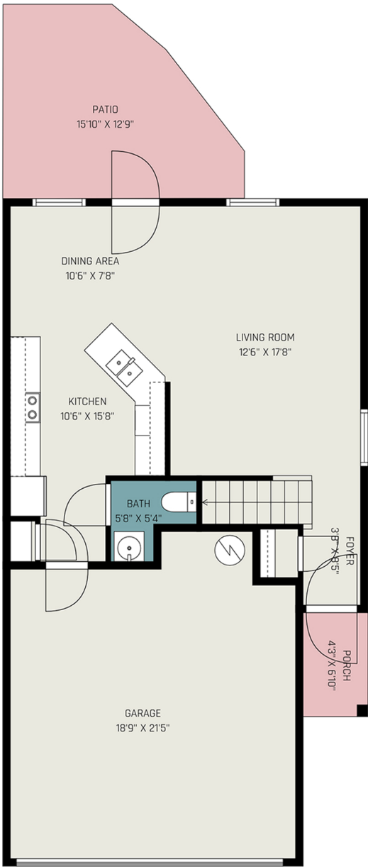
First Floor
