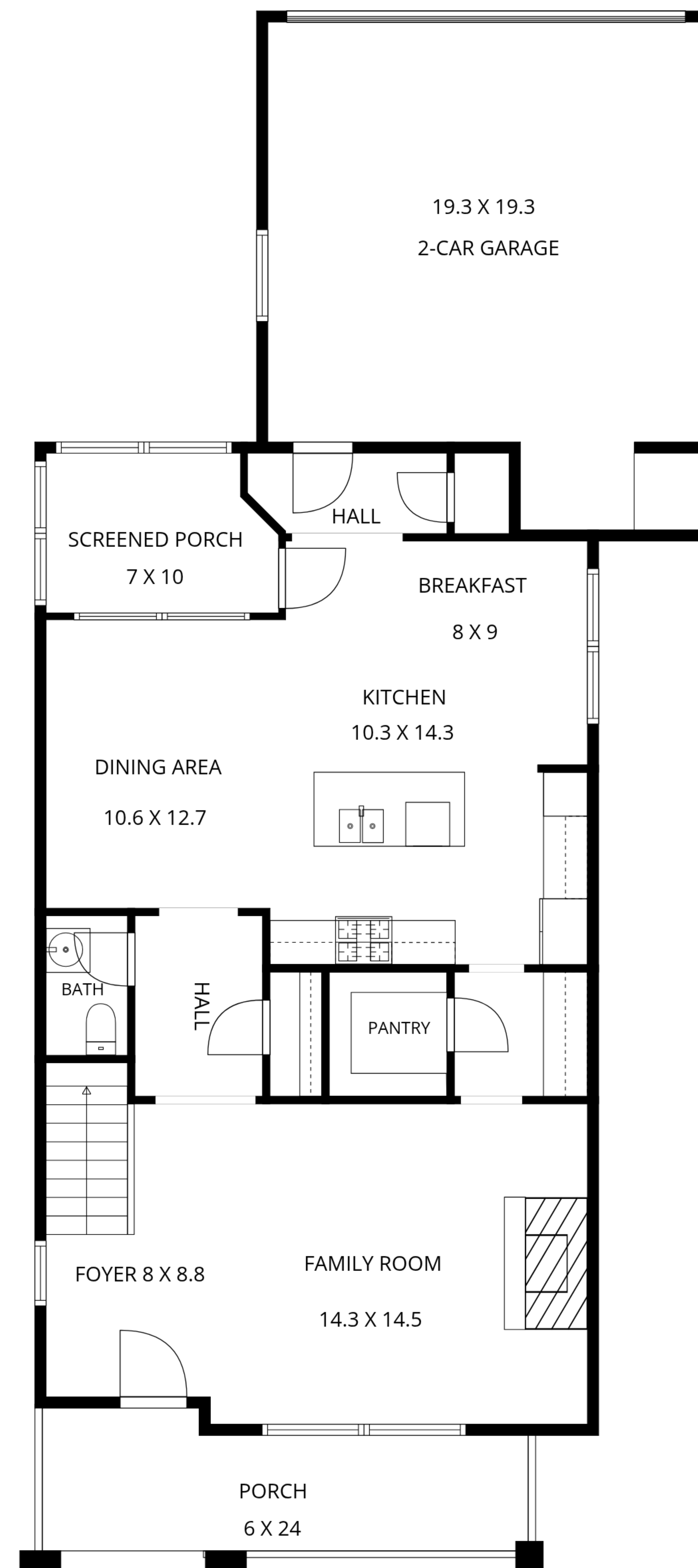
1ST FLOOR
