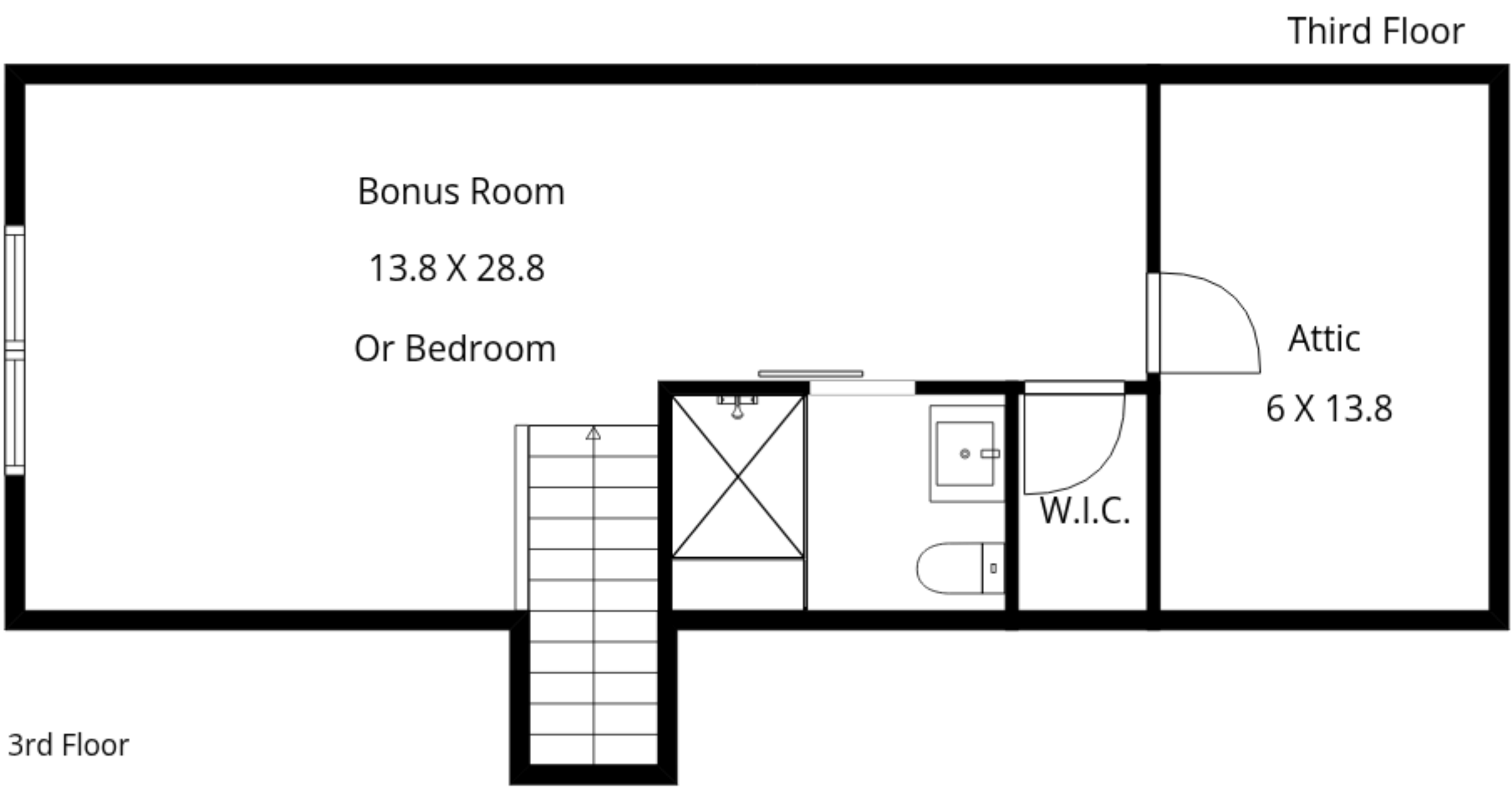
3rd Floor
