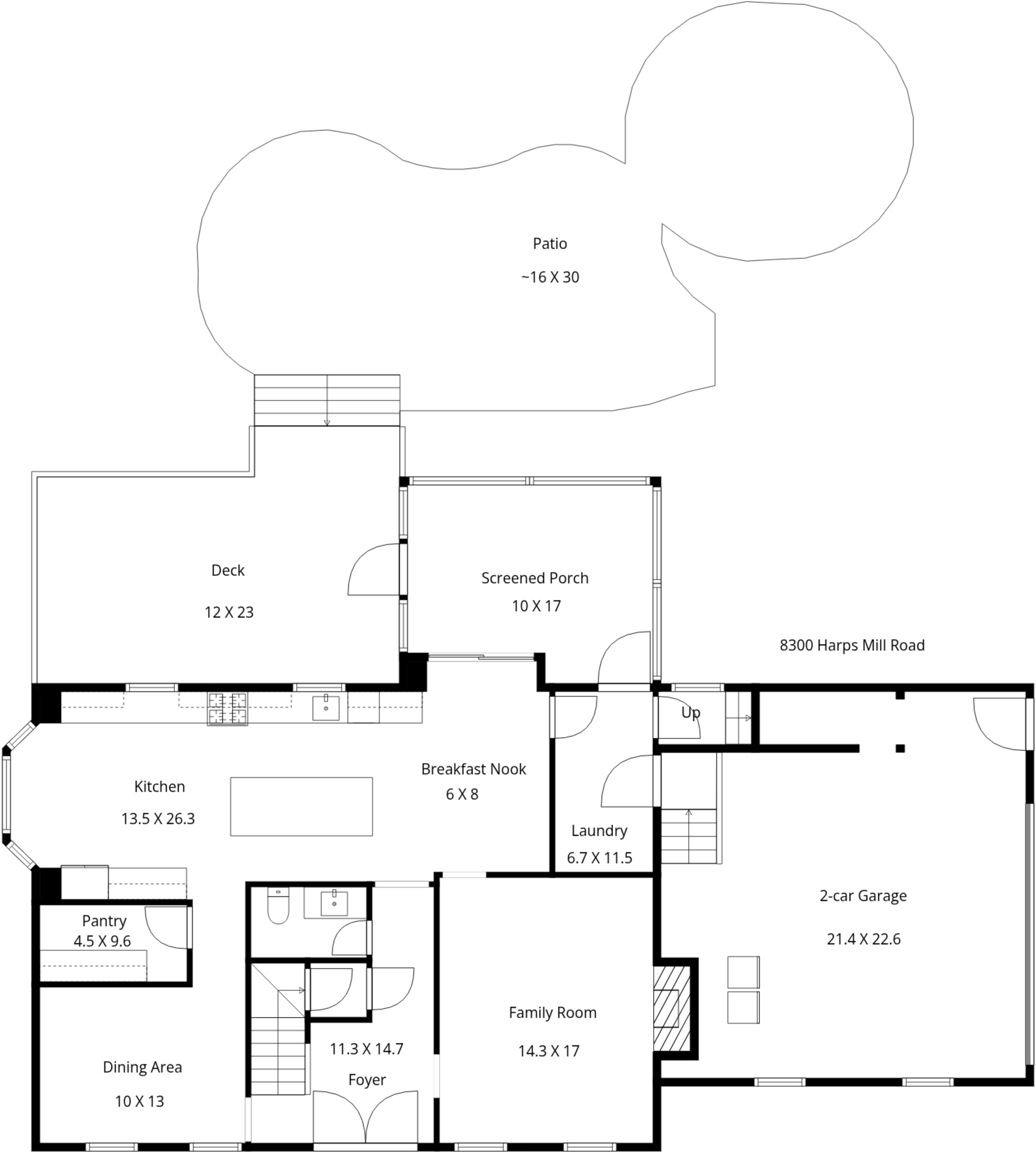
1st Floor
