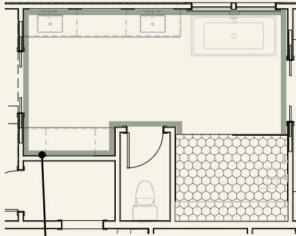
WAINSCOTING EXTENTS
