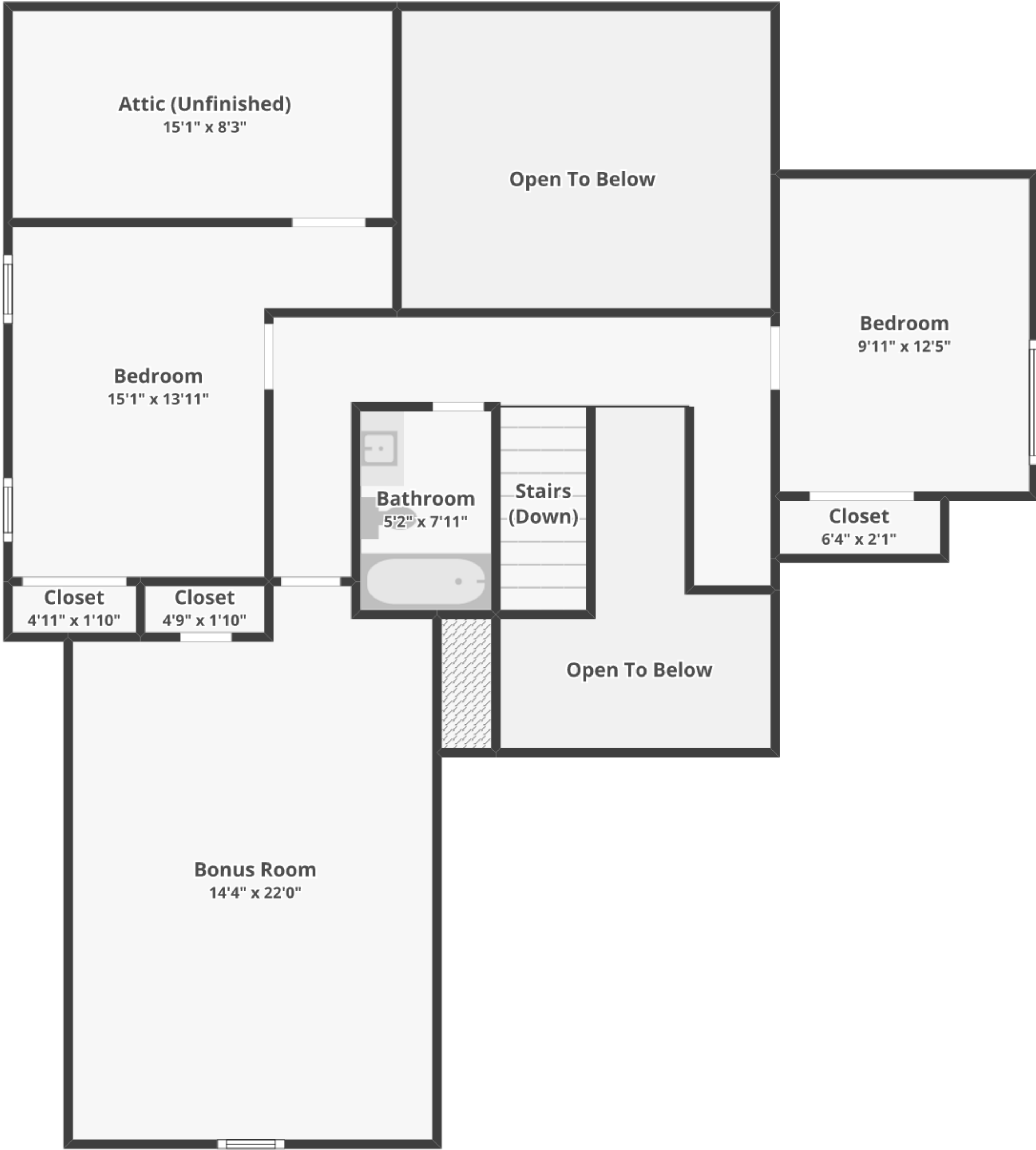
FLOOR 2
