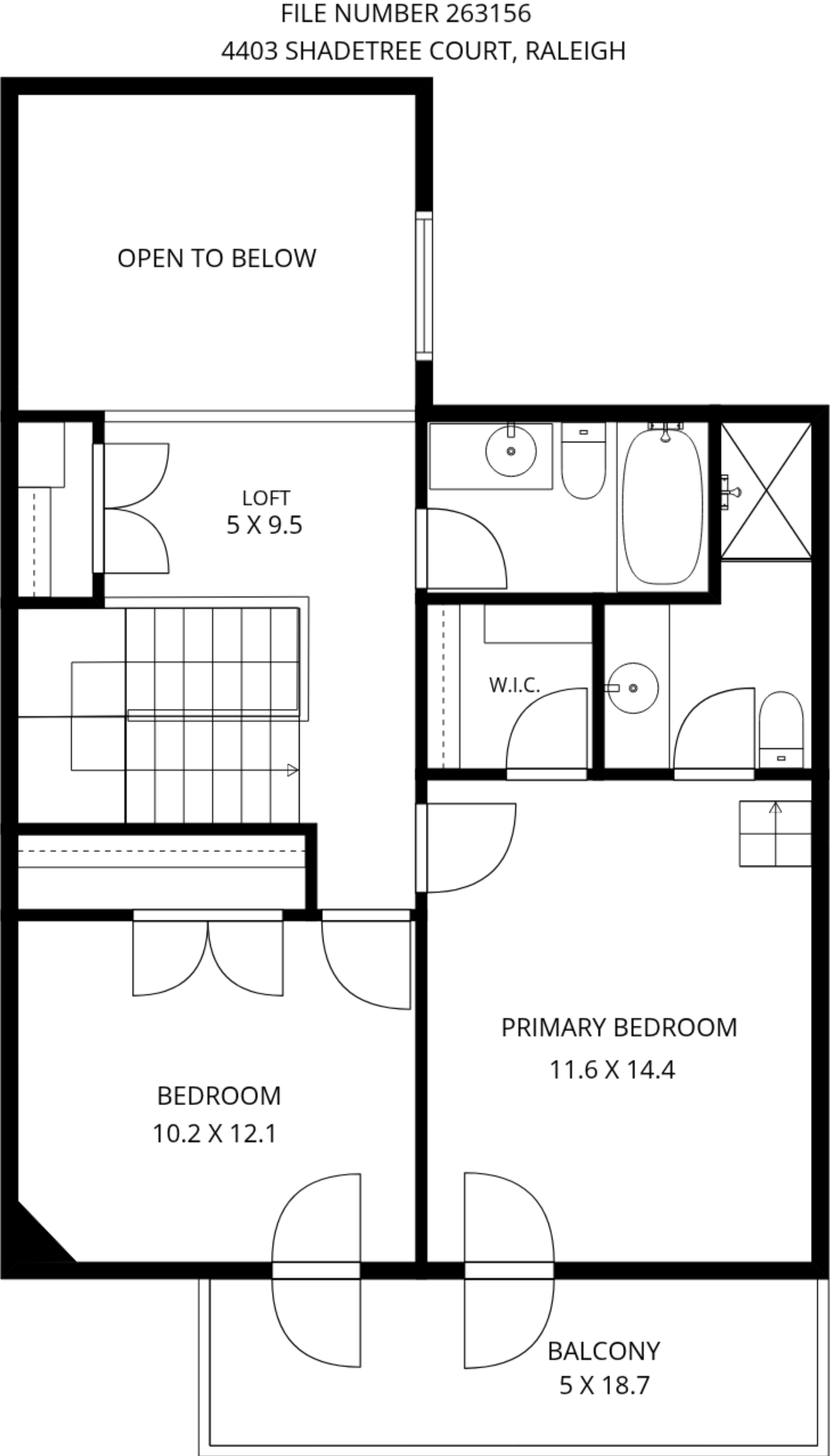
2ND FLOOR
