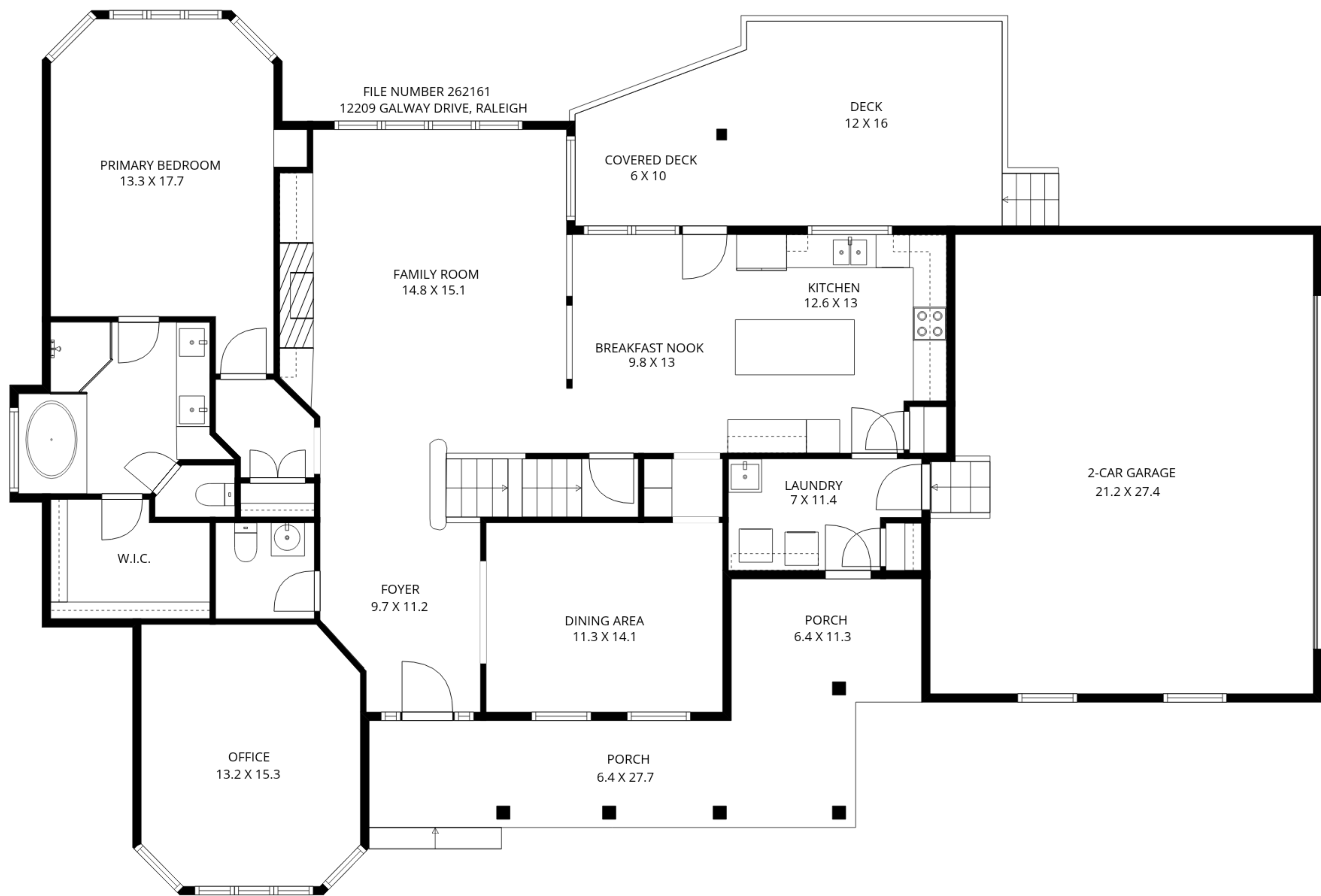
1ST FLOOR
