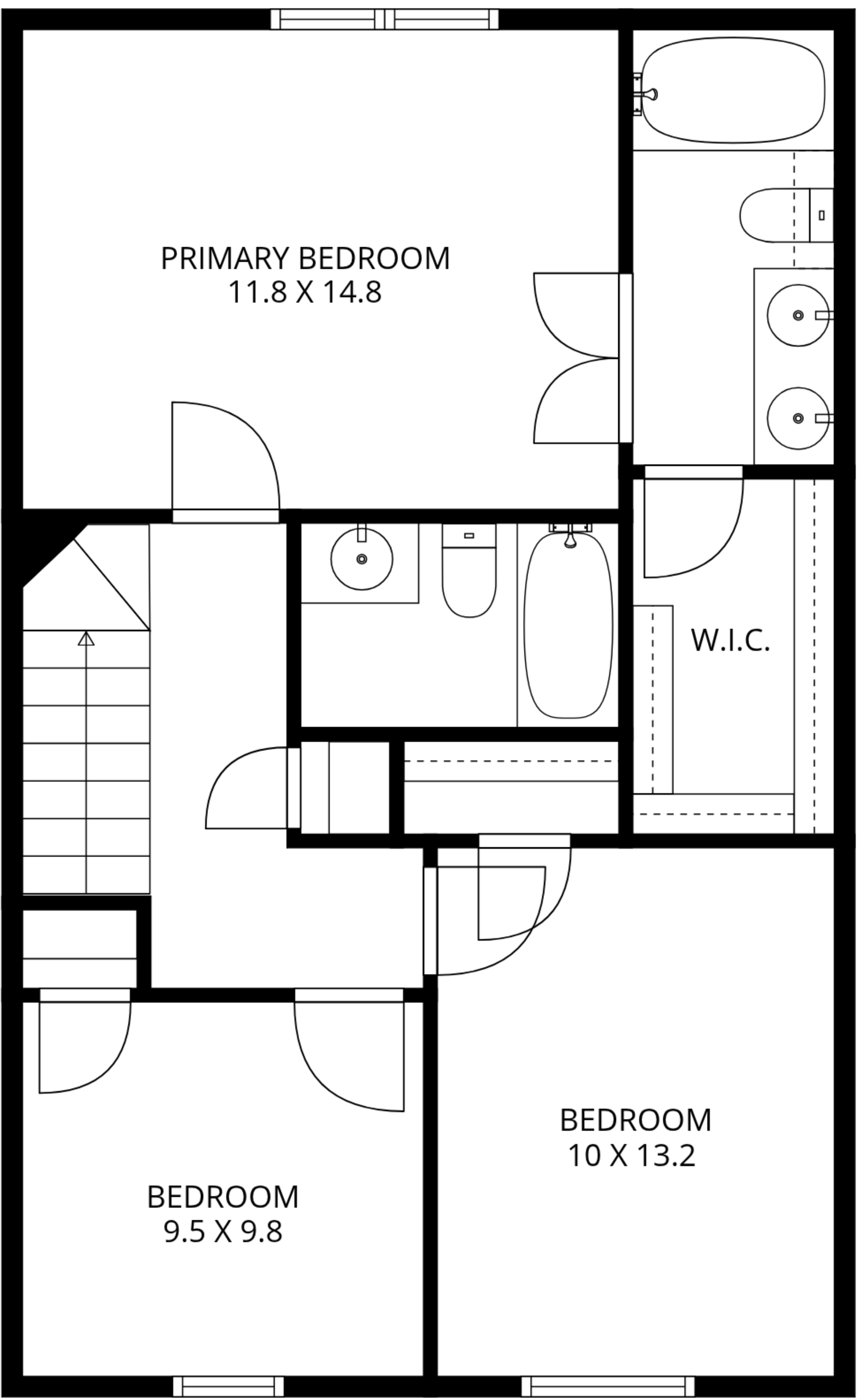
3RD FLOOR
