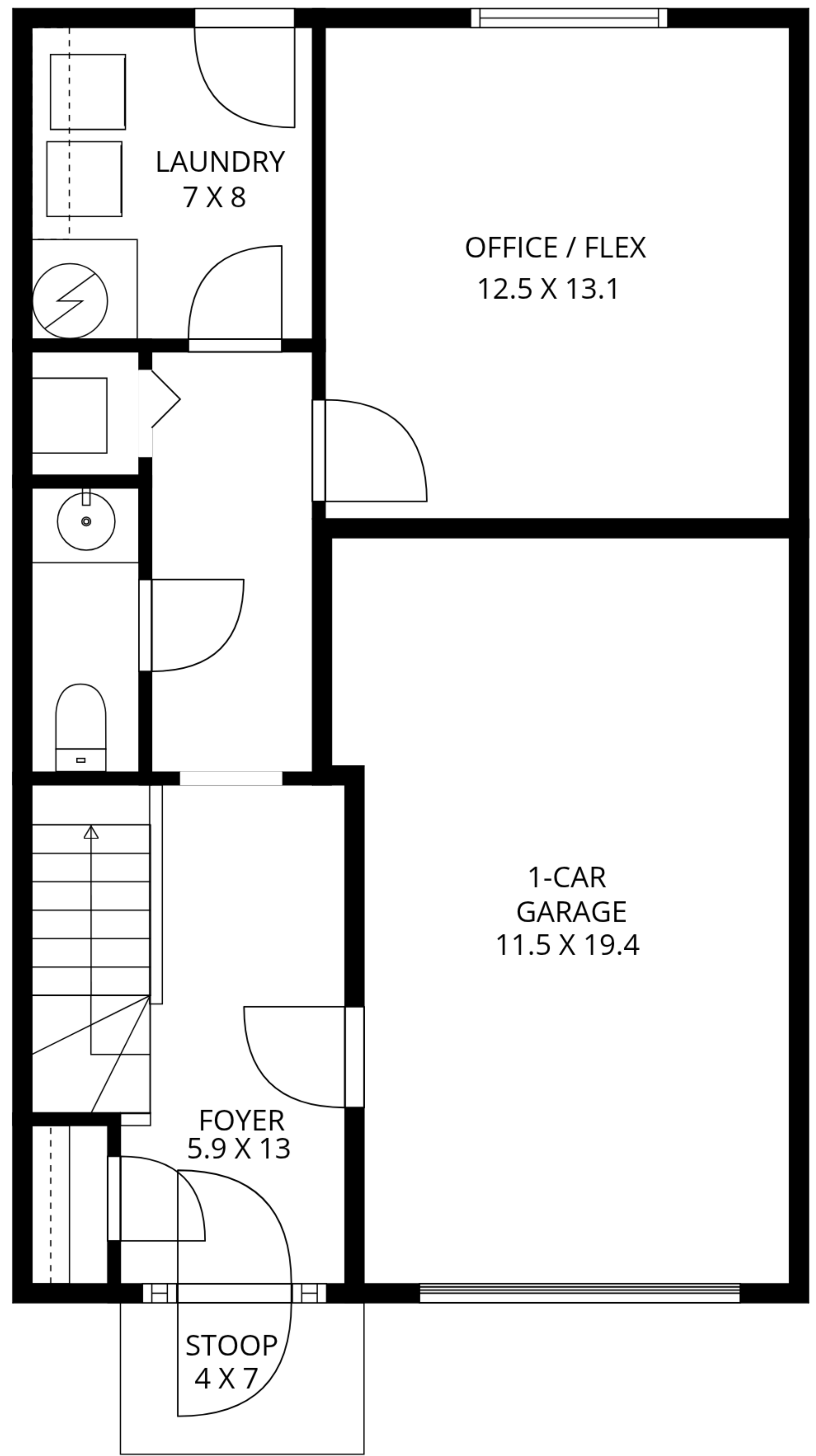
1ST FLOOR
