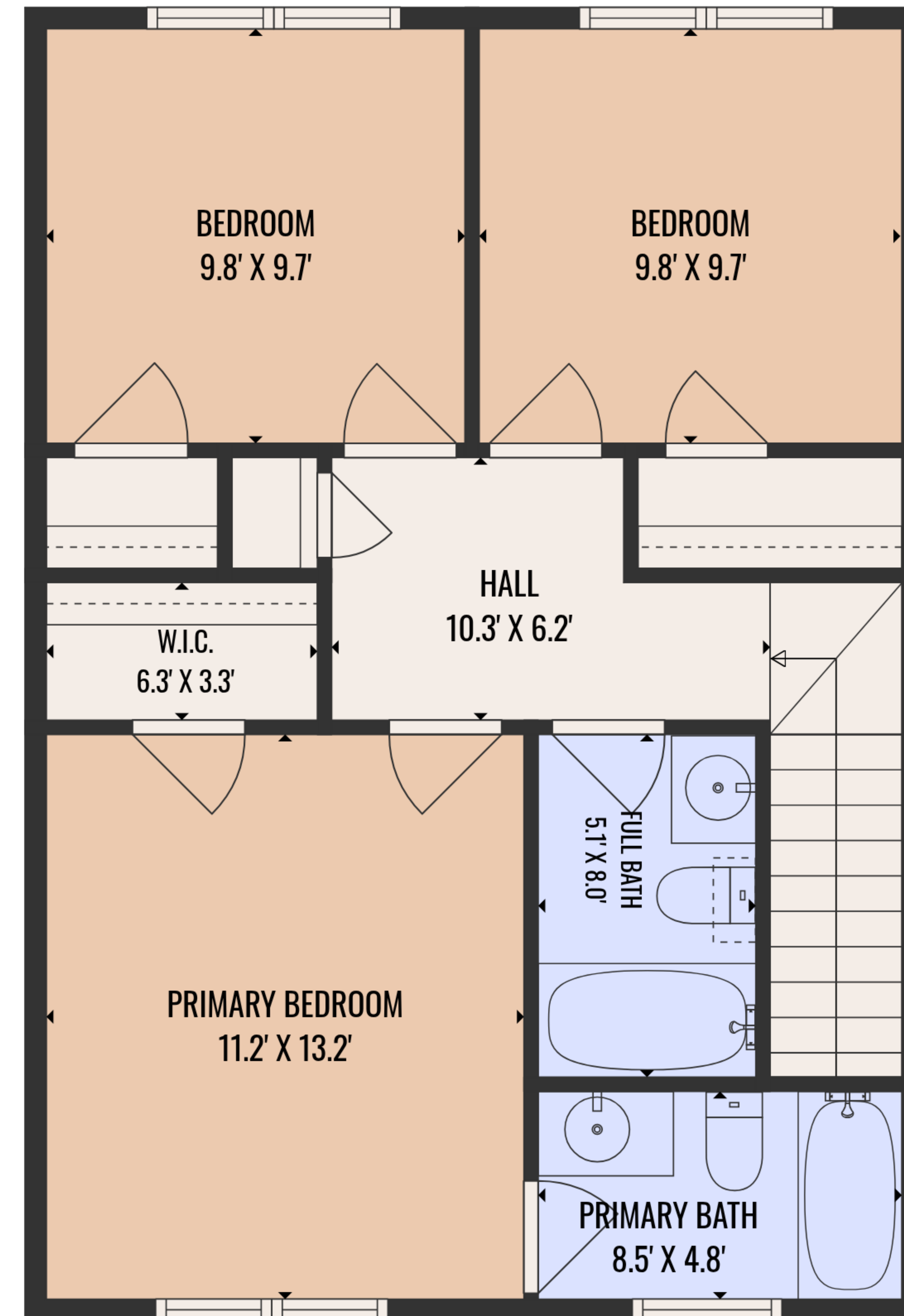
2ND FLOOR
