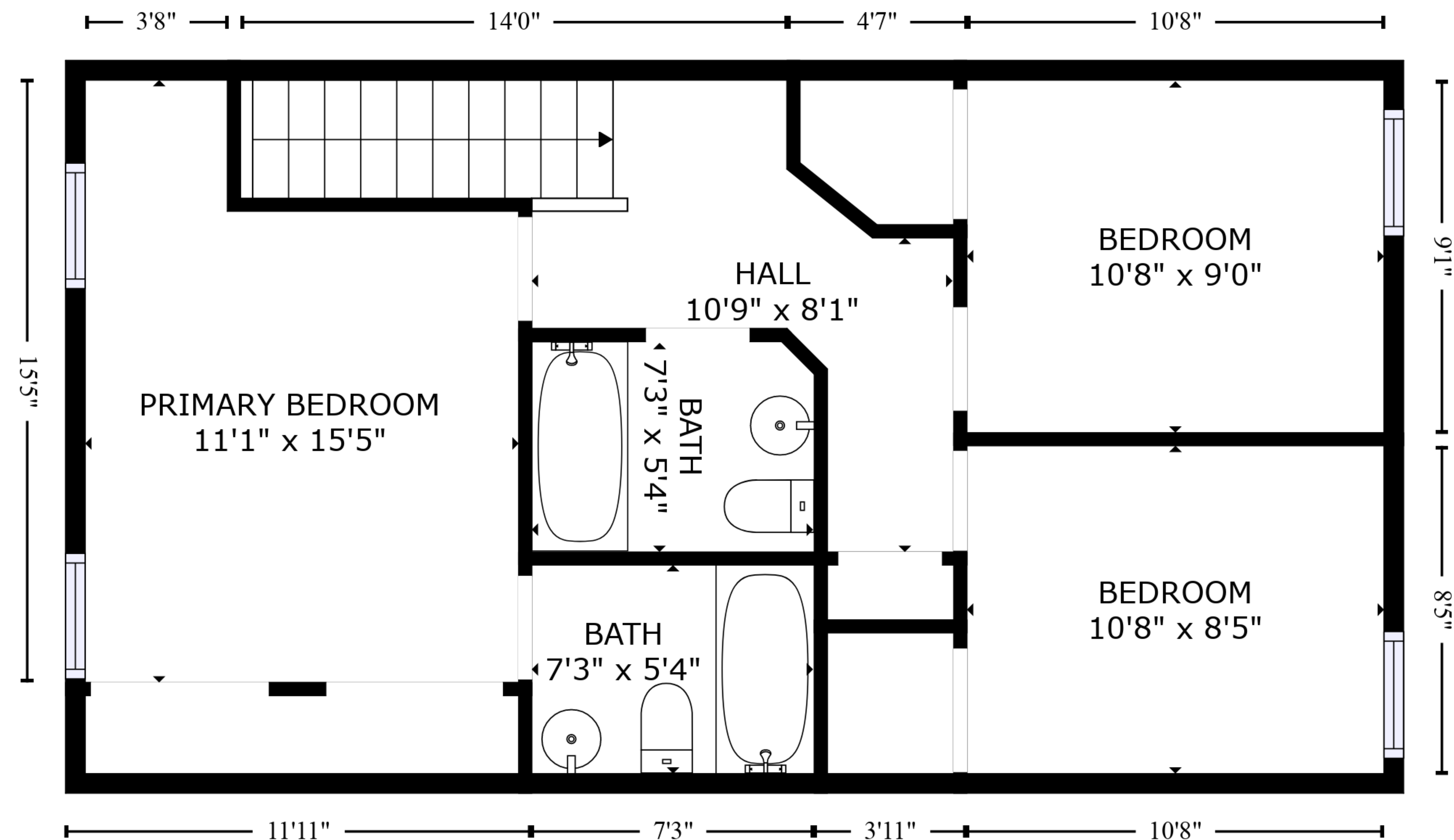
FLOOR 2
