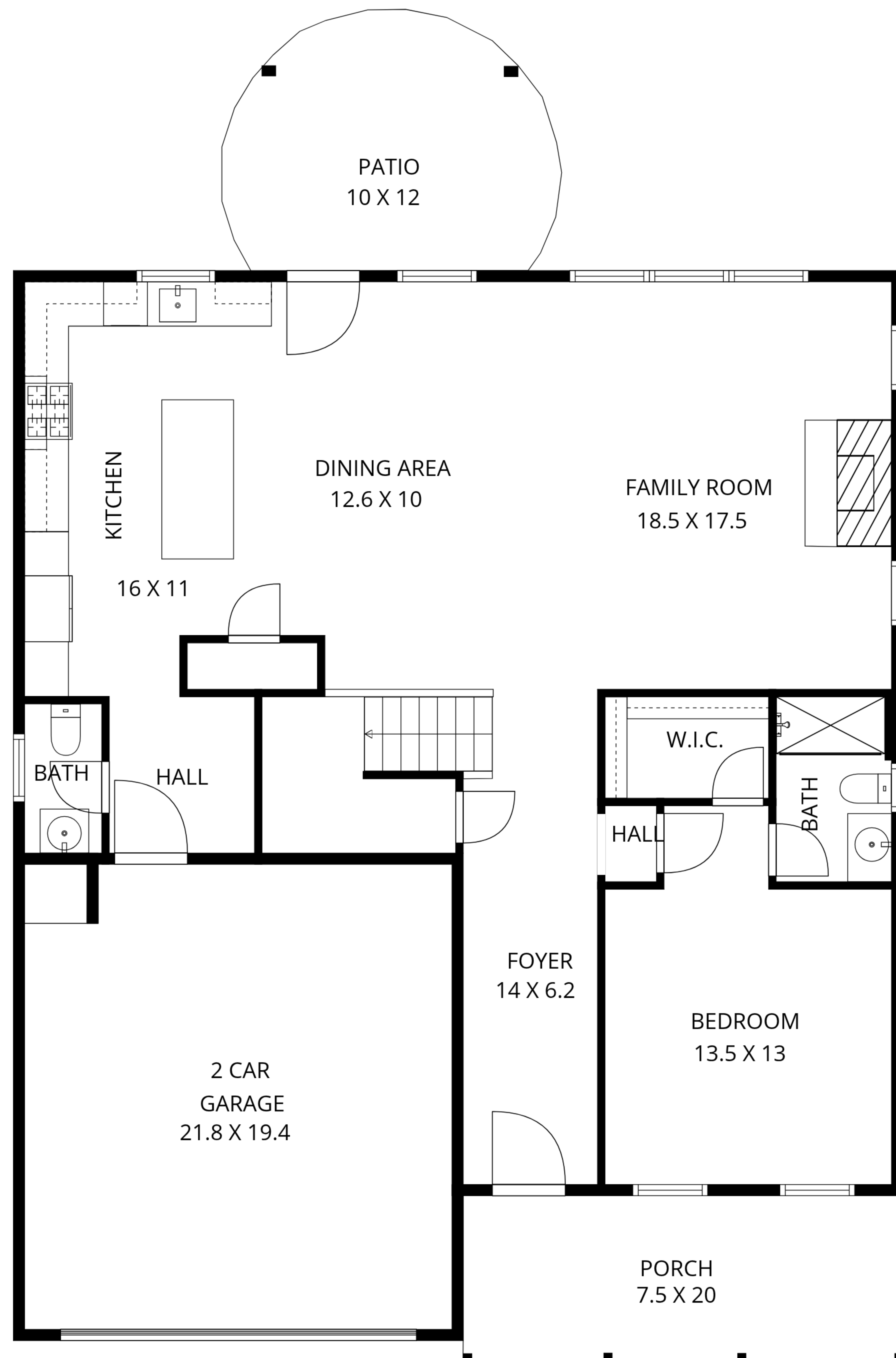
1ST FLOOR
