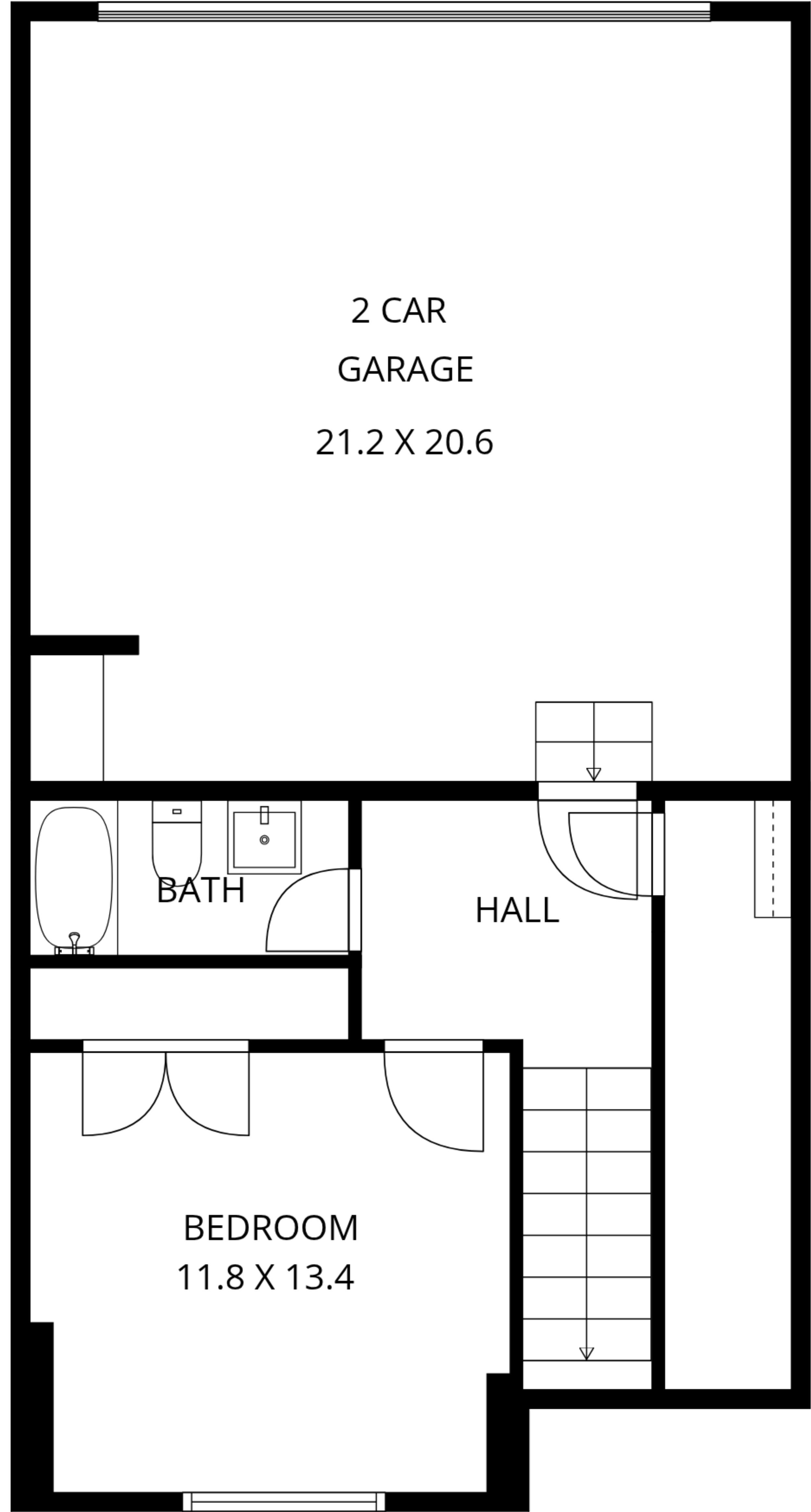
1ST FLOOR
