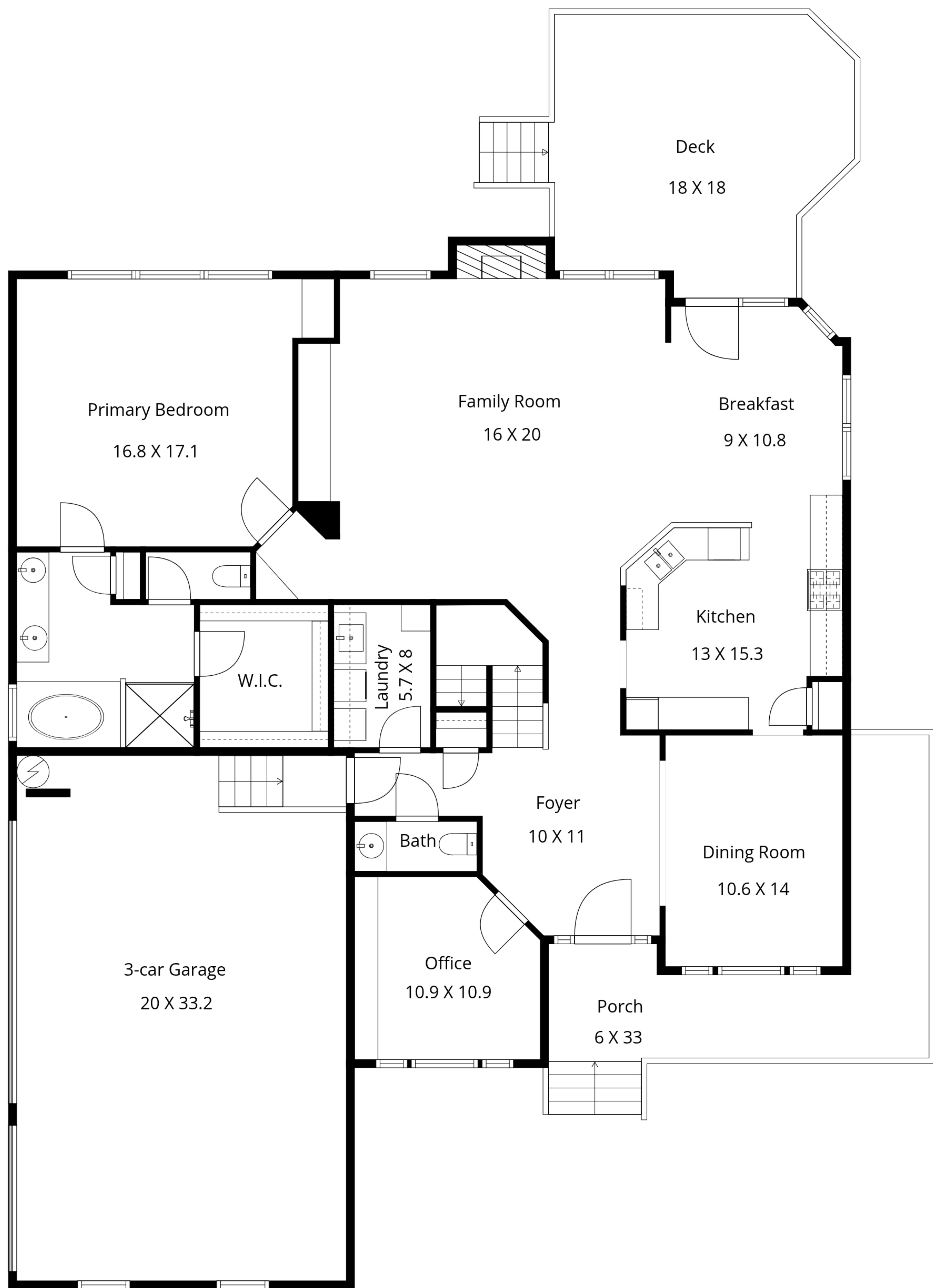
1st Floor
