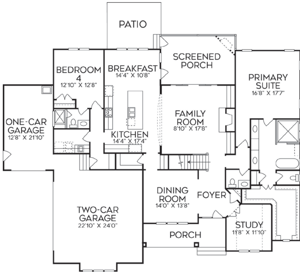
FIRST FLOOR
