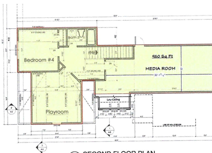
1 SECOND FLOOR PLAN SCALE: 3/16" = 1'-0"
