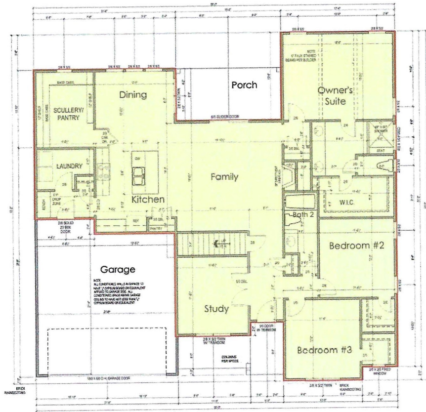
1 FIRST FLOOR PLAN SCALE: 3/16" = 1'-0"
