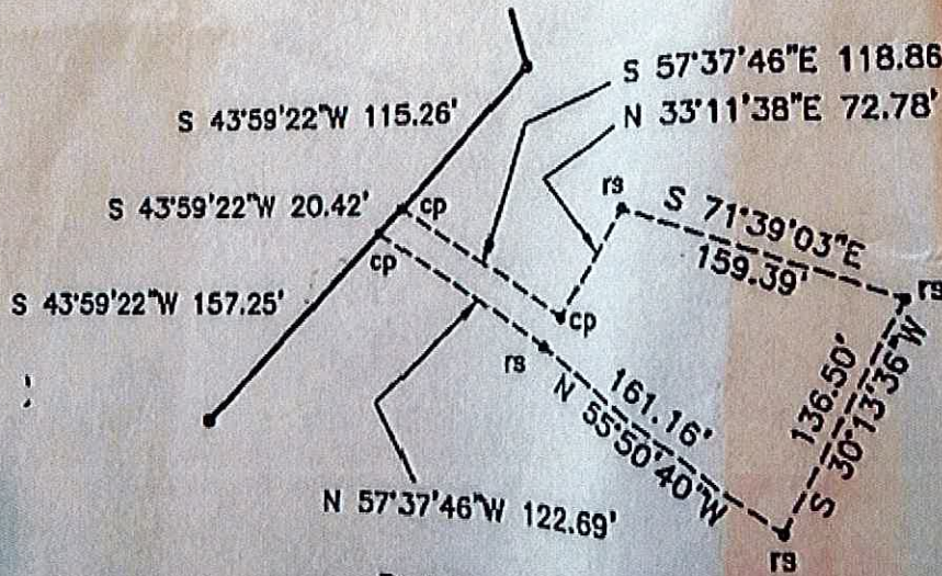
Detail A Drainfield Easement for Lot 1
