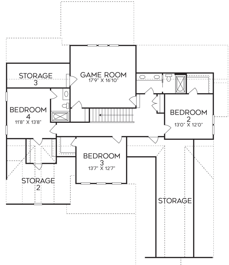
SECOND FLOOR
