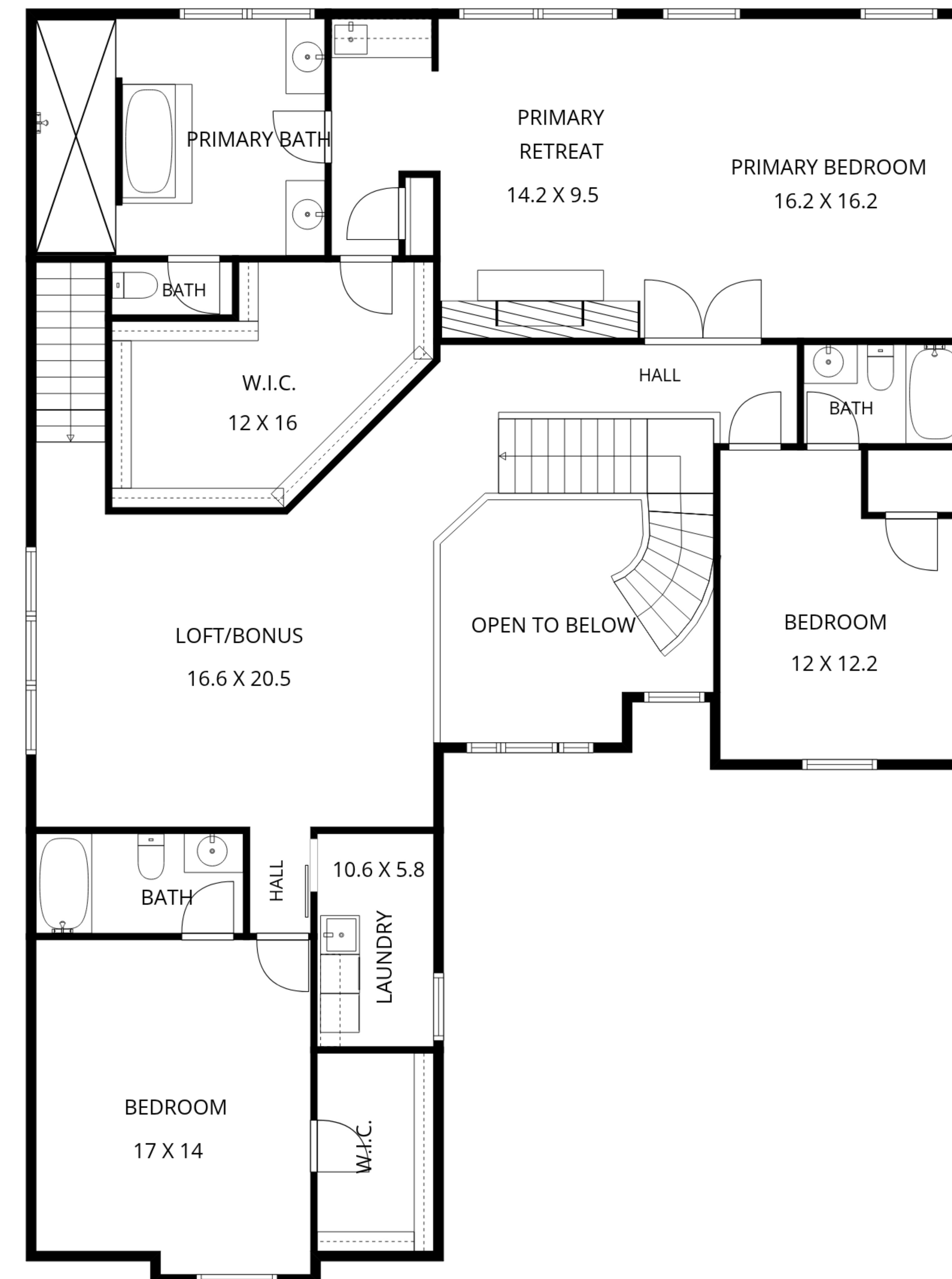
2ND FLOOR
