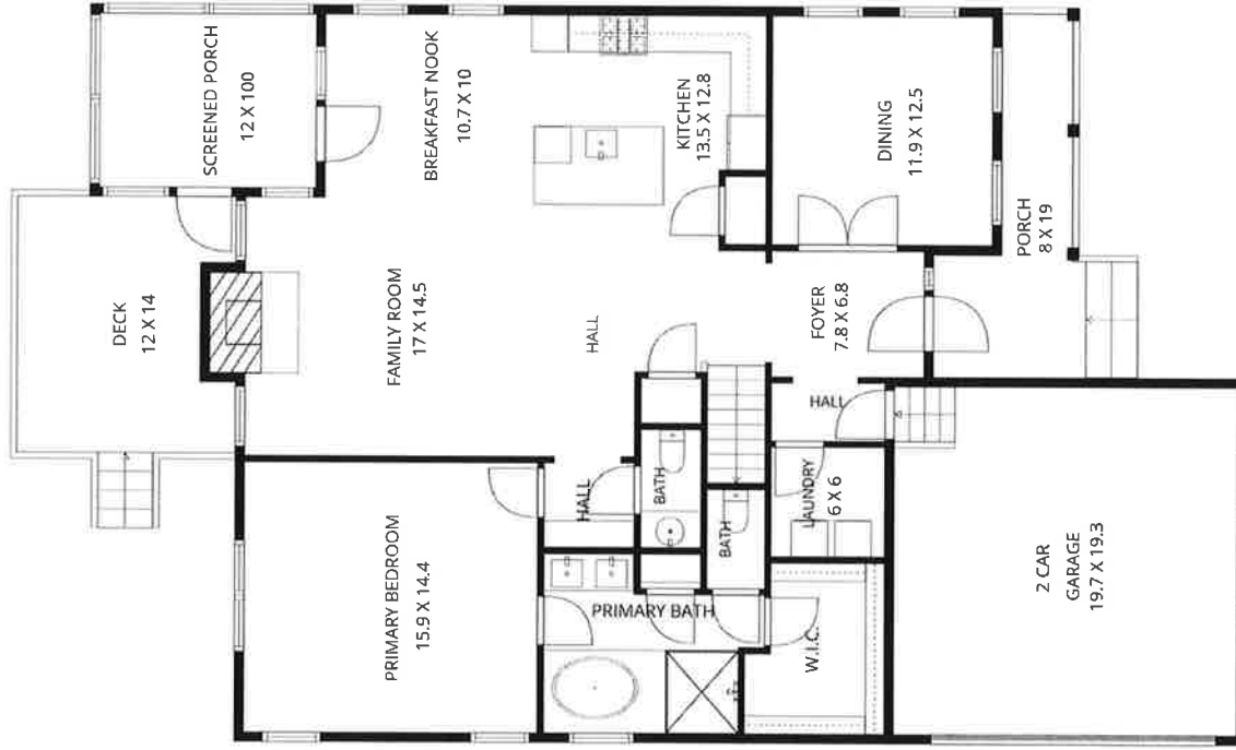
1ST FLOOR
