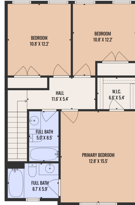
2ND FLOOR
