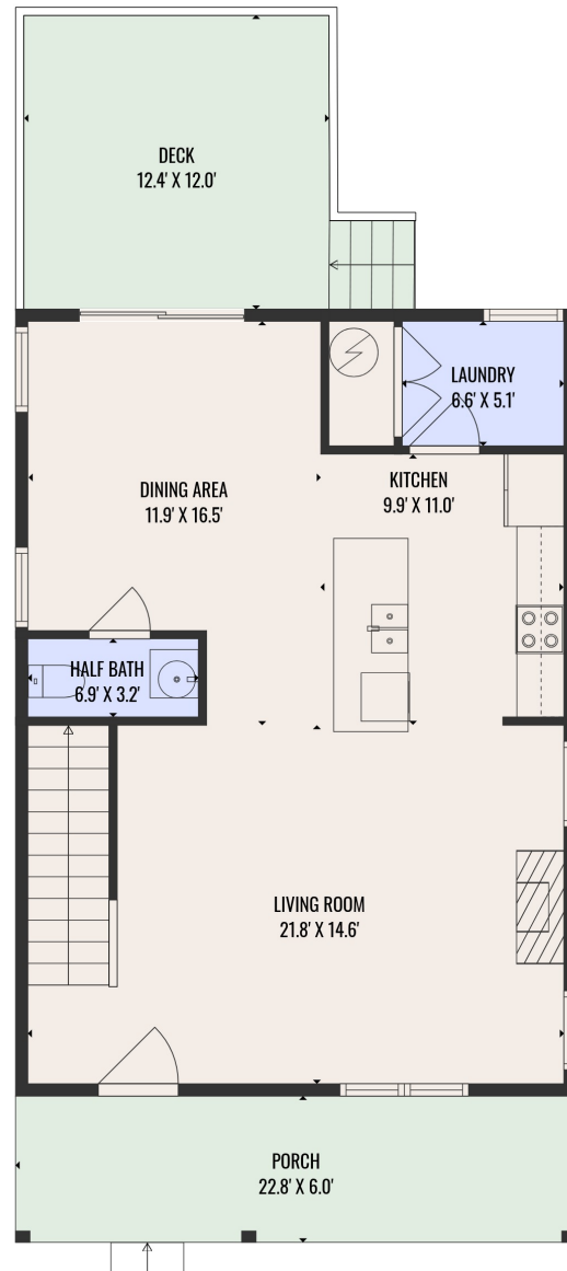
1ST FLOOR
