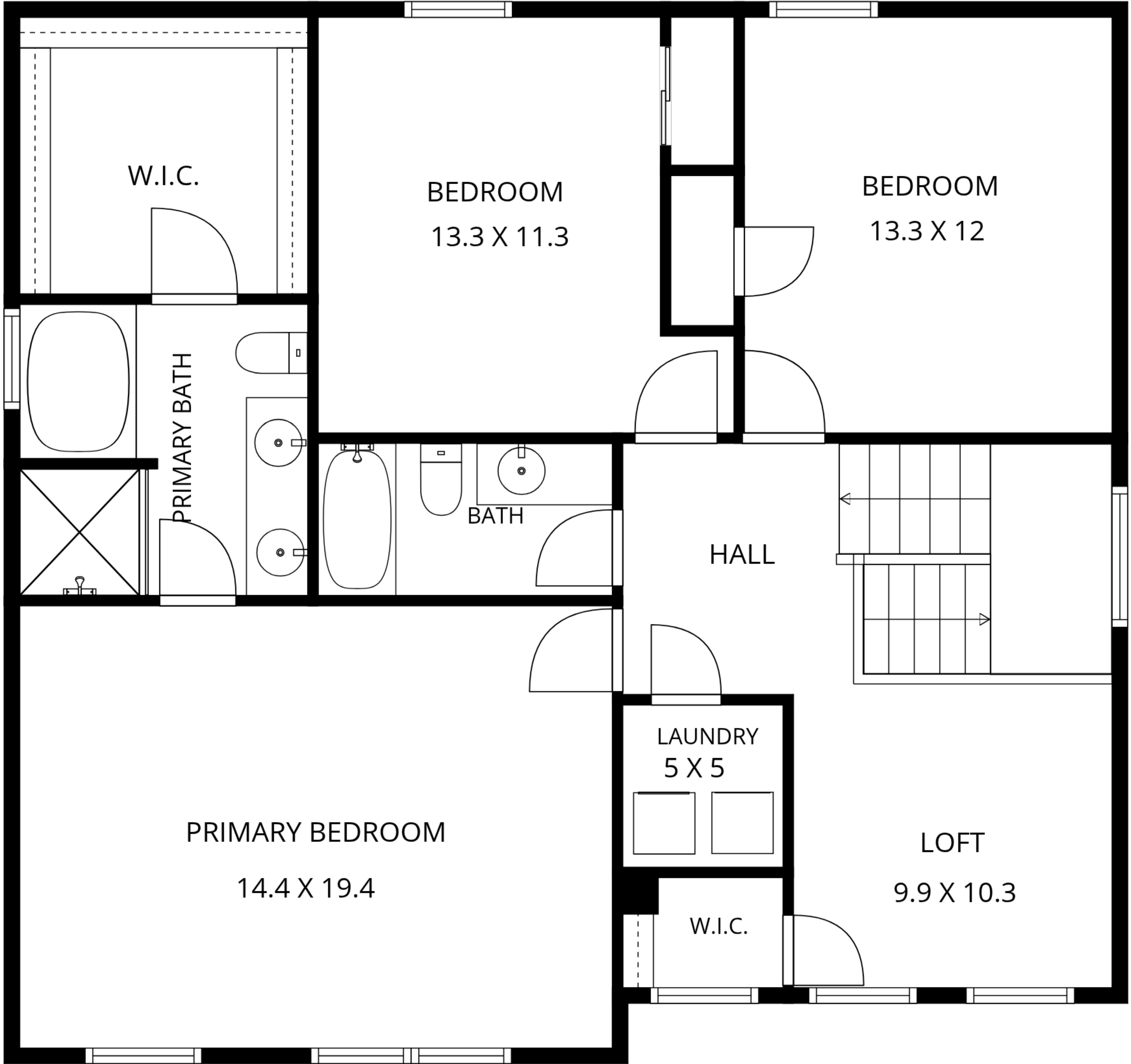
2ND FLOOR
