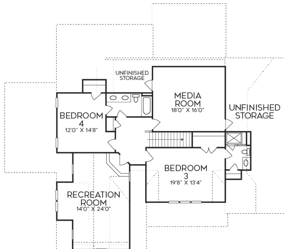
SECOND FLOOR
