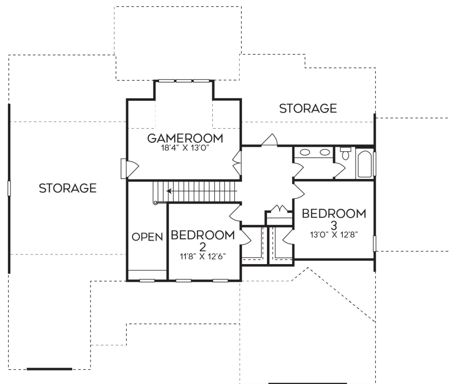
SECOND FLOOR
