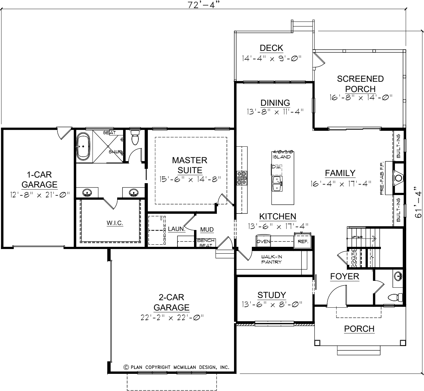
First Floor
