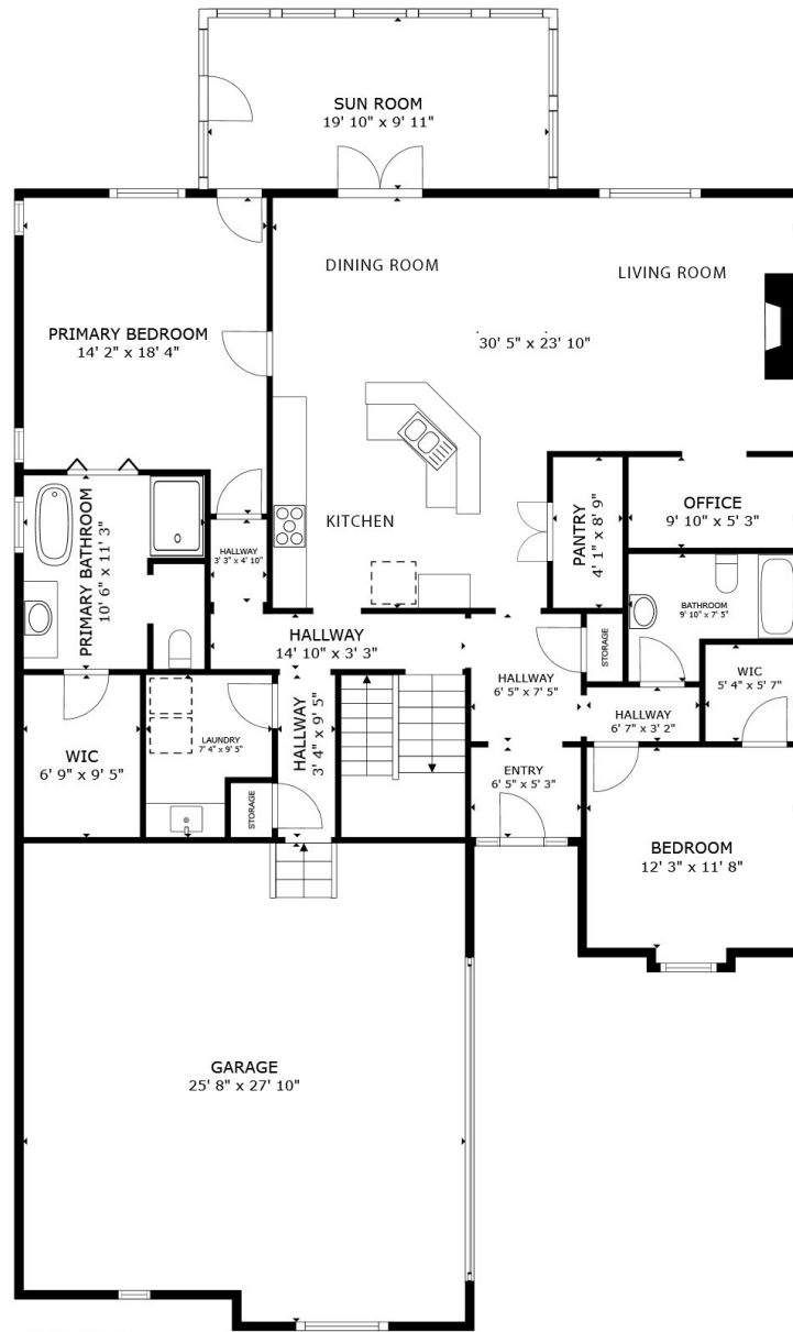
FLOOR 1 1,964 SQ.FT.
