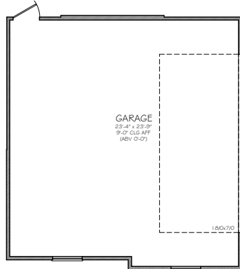
OPTION: SIDE ENTRY GARAGE ADDS 112 UNHEATED SQ. FT. REQUIRES ELEVATION C
