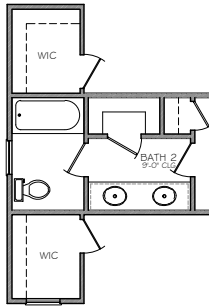
OPTION: BATH 2/BED 2 & 3 CLOSET BUMP OUT 5'-4" ADDS 104 HEATED SQ. FT. INCLUDED WITH ELEVATION B & C
