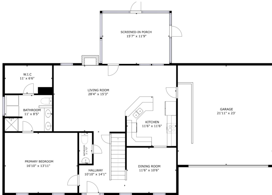
FLOOR 1 1,219 SQ.FT.
