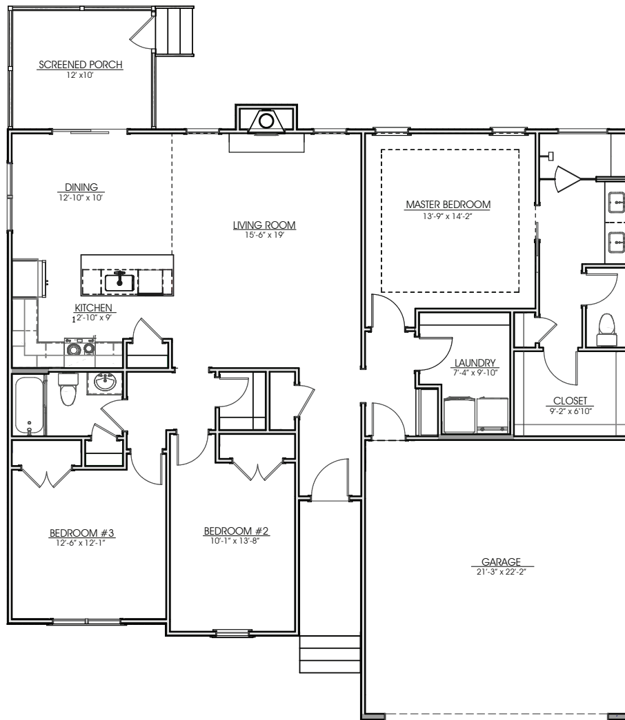
FIRST FLOOR
