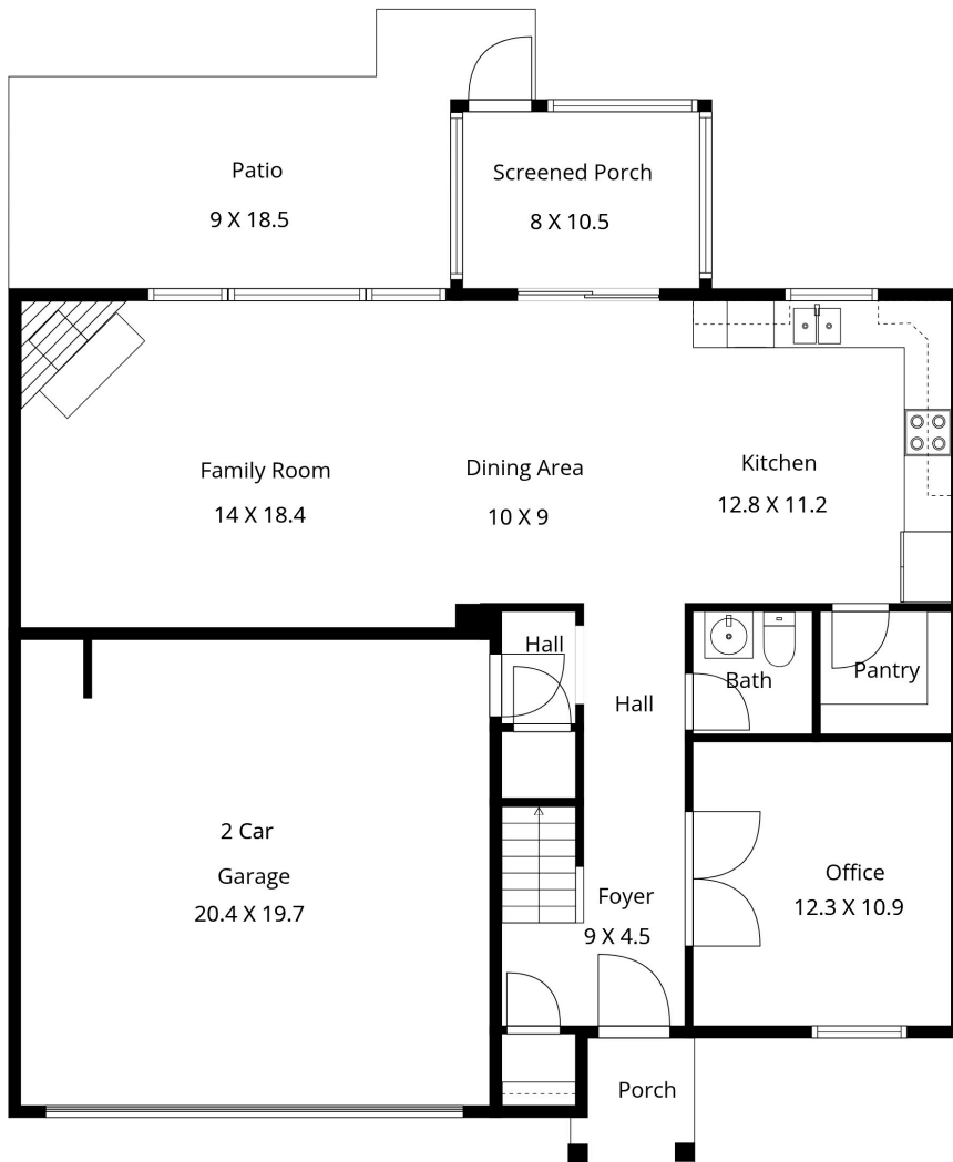
1st Floor
