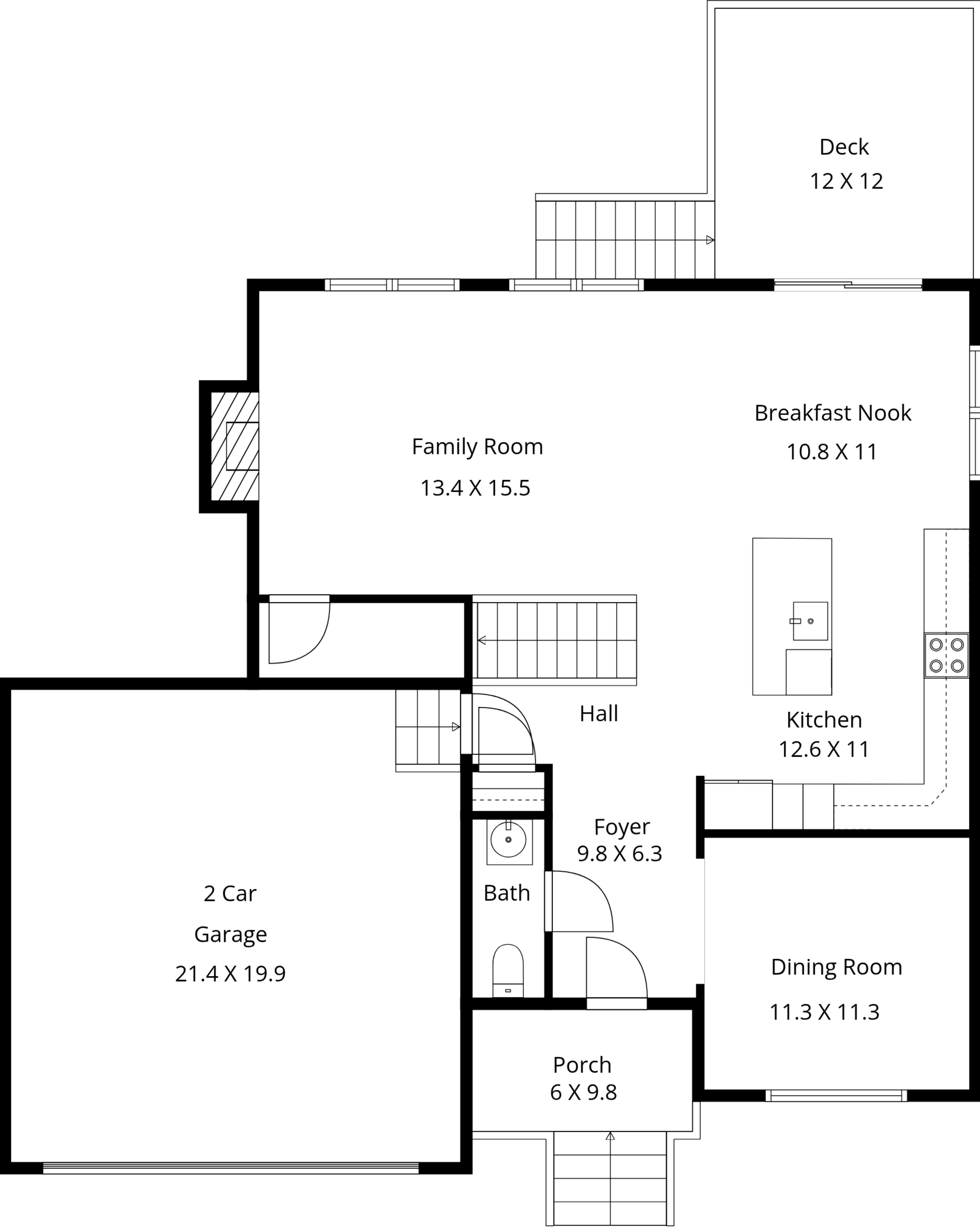
1st Floor
