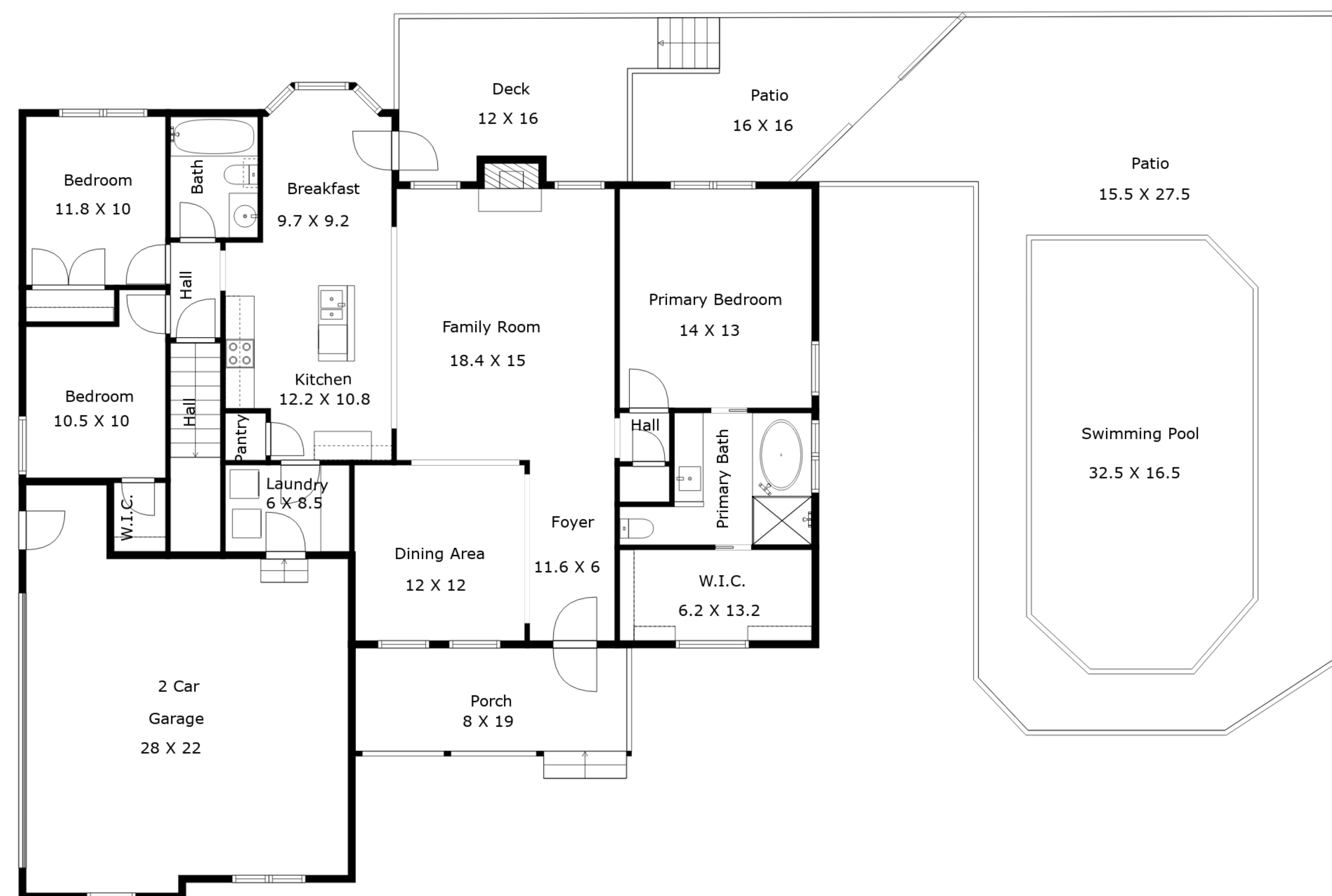
Floor 1
