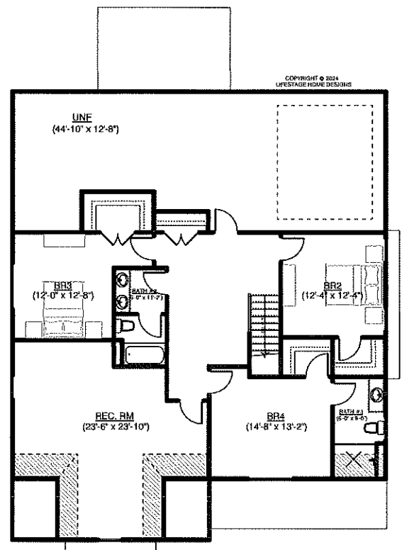
2ND FLOOR
