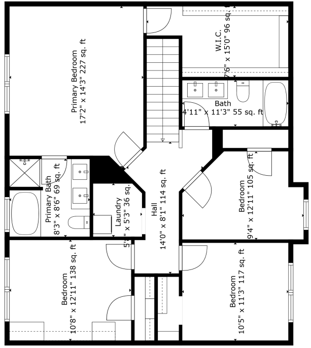
Floor 2
