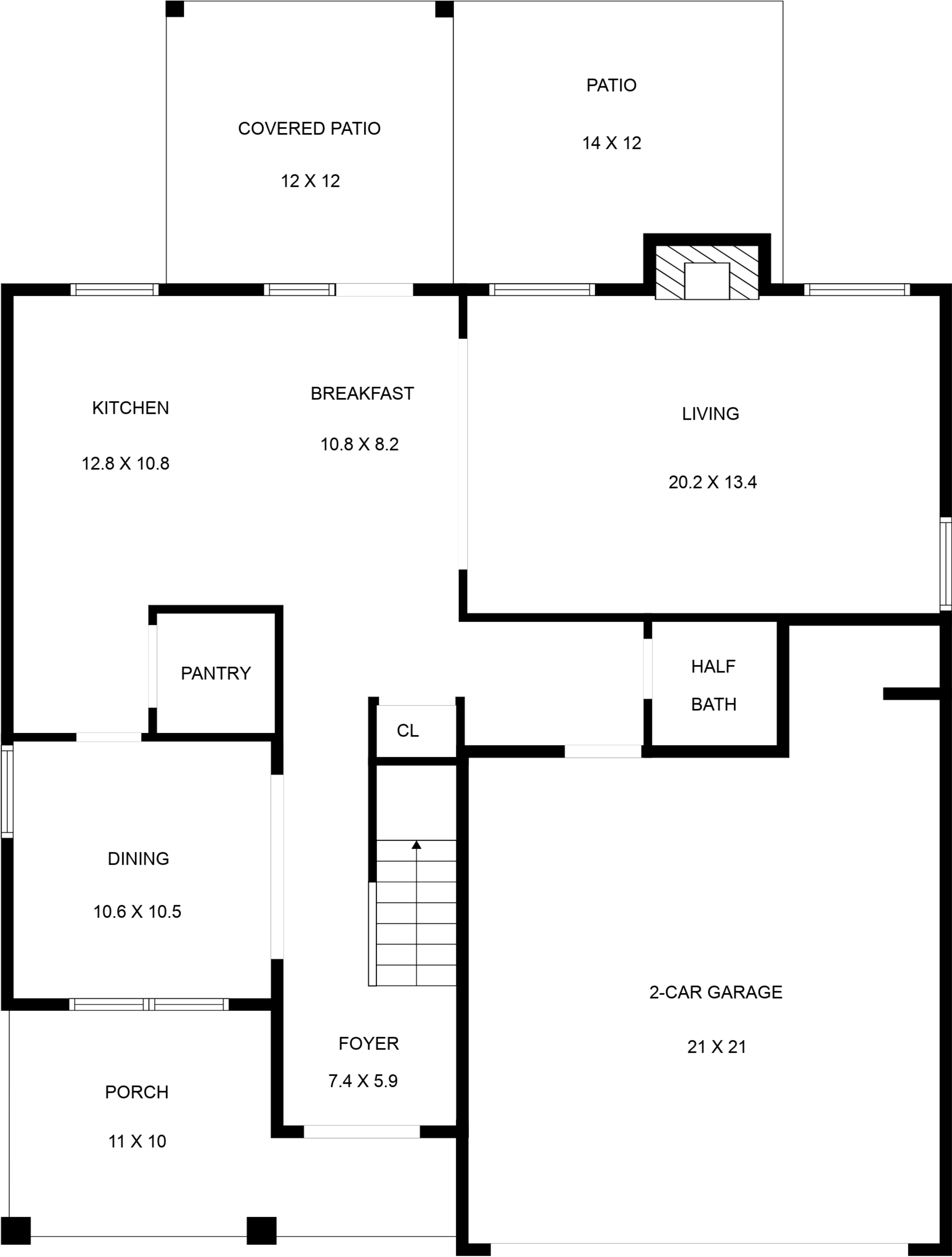
FLOOR 1
