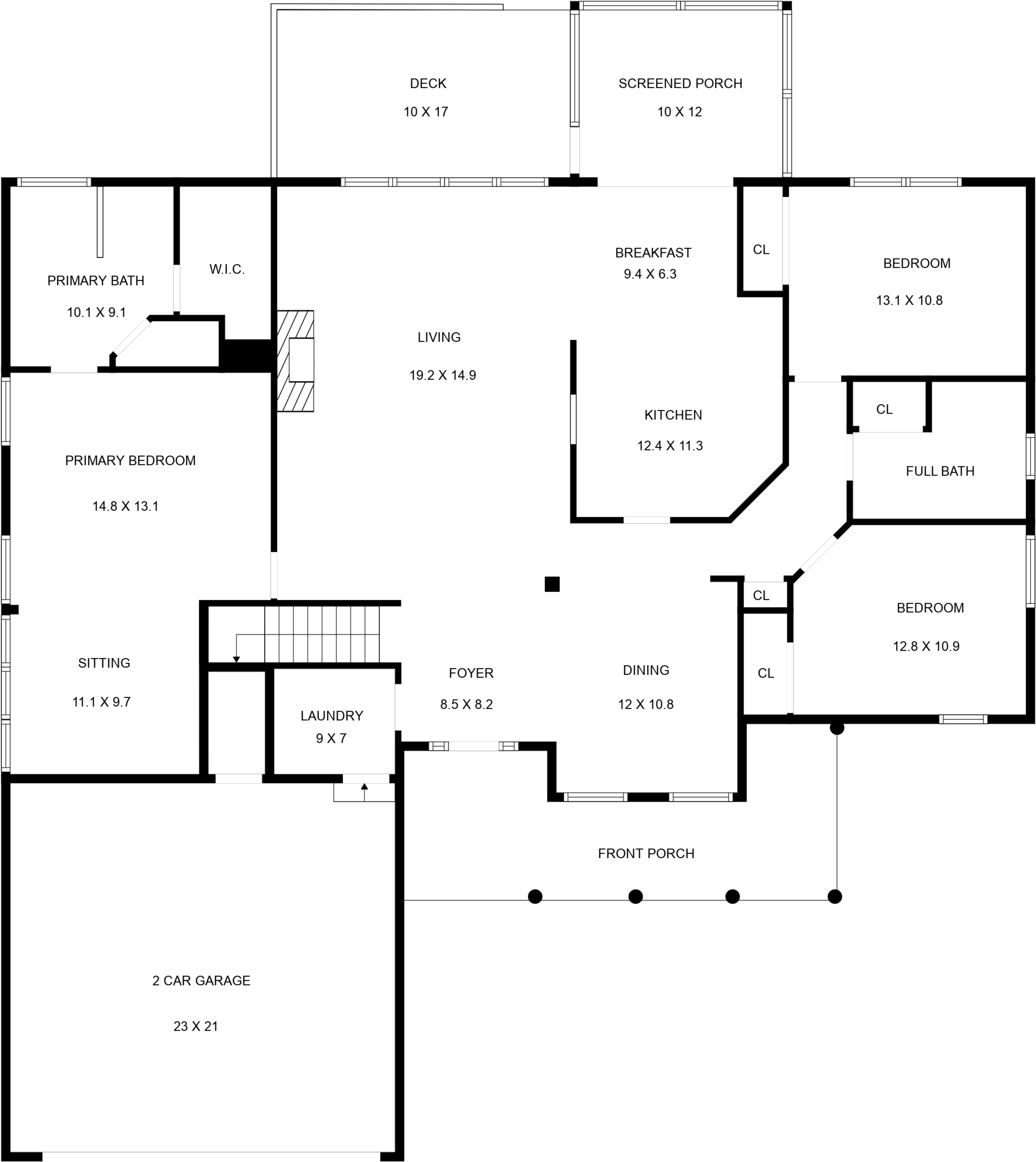
FLOOR 1
