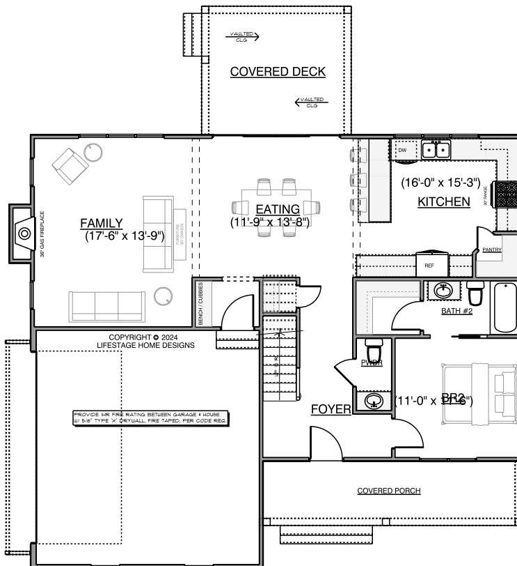
1ST FLOOR
