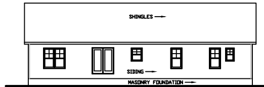
REAR ELEVATION
