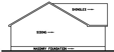
LEFT ELEVATION
