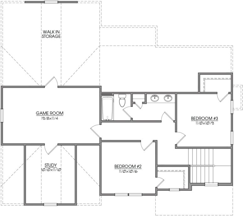
SECOND FLOOR
