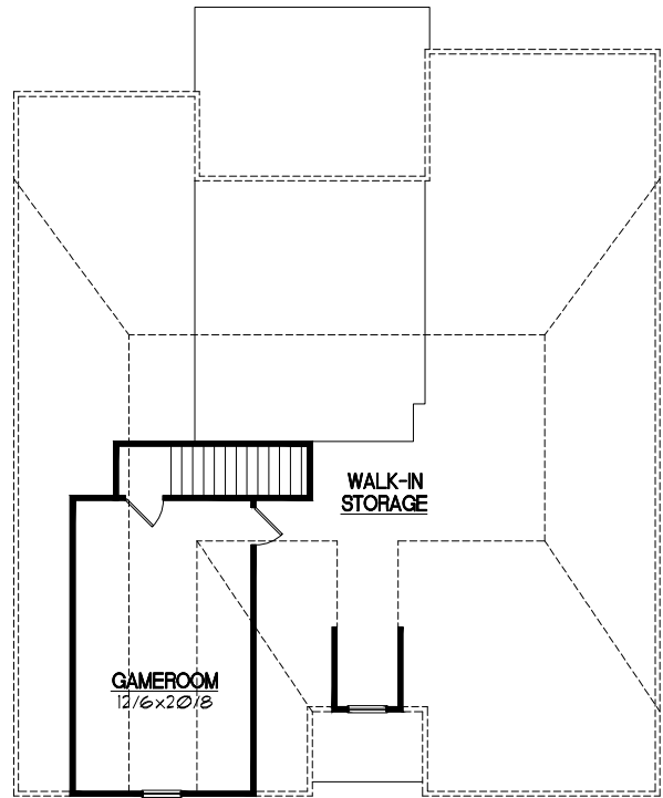
Second Floor
