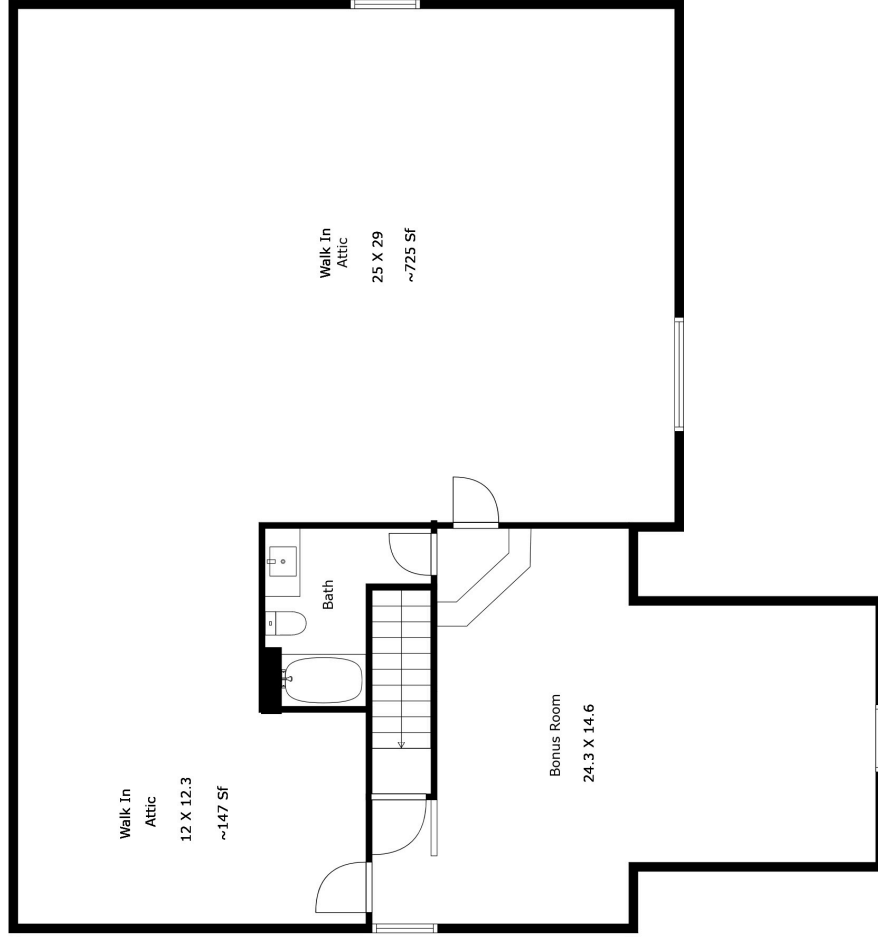
Floor 2
